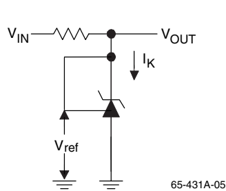
Figure 1. Test Circuit for V_{KA} = V_{REF} , V_{OUT} = V_{KA} = V_{REF}
