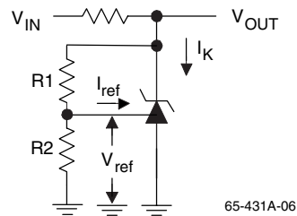
Figure 2. Test Circuit for V_{KA} > V_{REF} , V_{OUT} = V_{KA} = V_{REF} \times (1 + R1/R2) + I_{REF} \times R1
