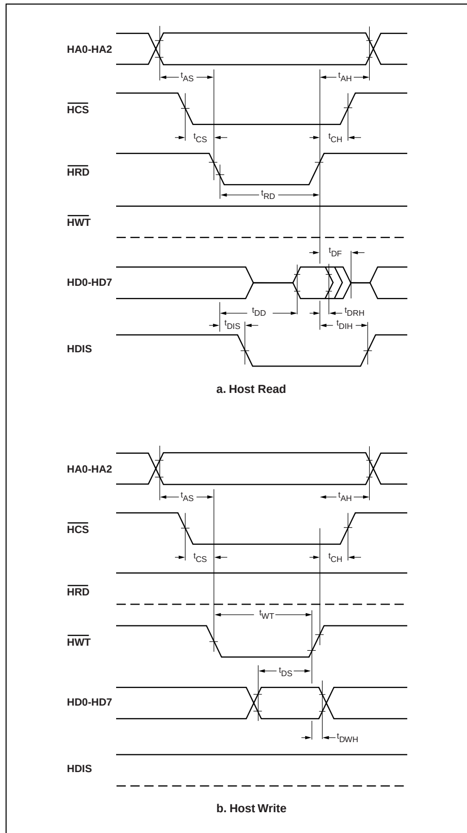
Figure 7-1. Timing Waveform
