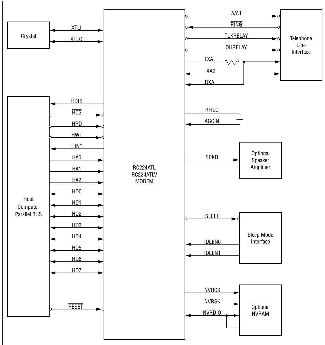
Figure 2-1. RC224ATLV Signals—Parallel Interface
