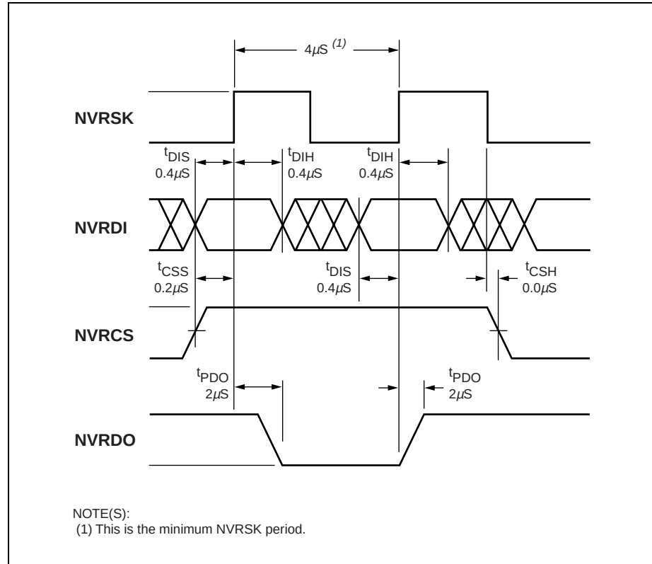
Figure 3-5. NVRAM Timing
