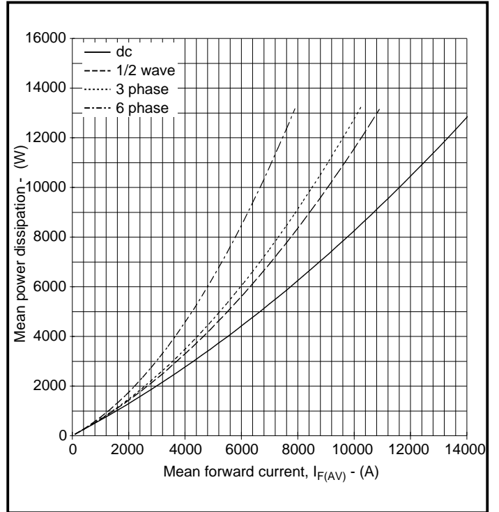
Fig. 3 Power dissipation
