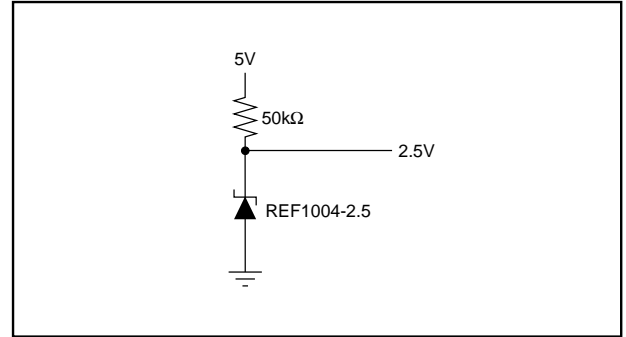
FIGURE 4. 2.5V Reference.
