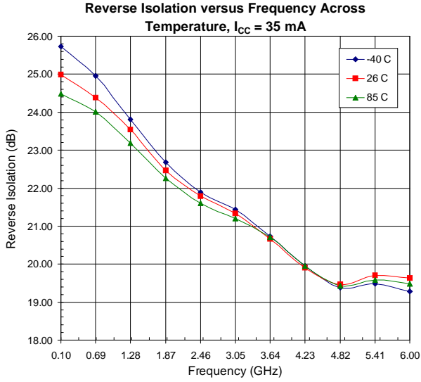
50 Ohms, 35 mA
