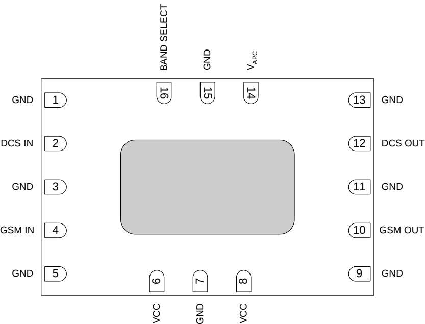
Pin Out Top View
