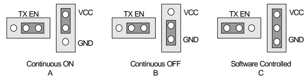
Figure 1. TX Enable Configuration
