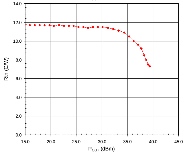
Thermal Resistance 460 MHz
