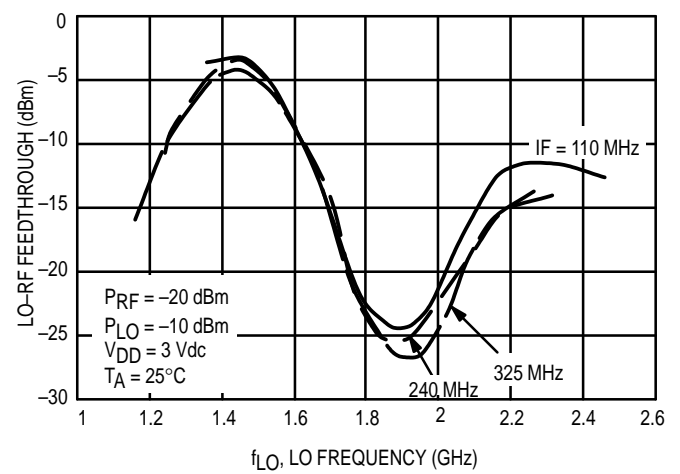
Figure 11. LO to RF Feedthrough versus LO Frequency
