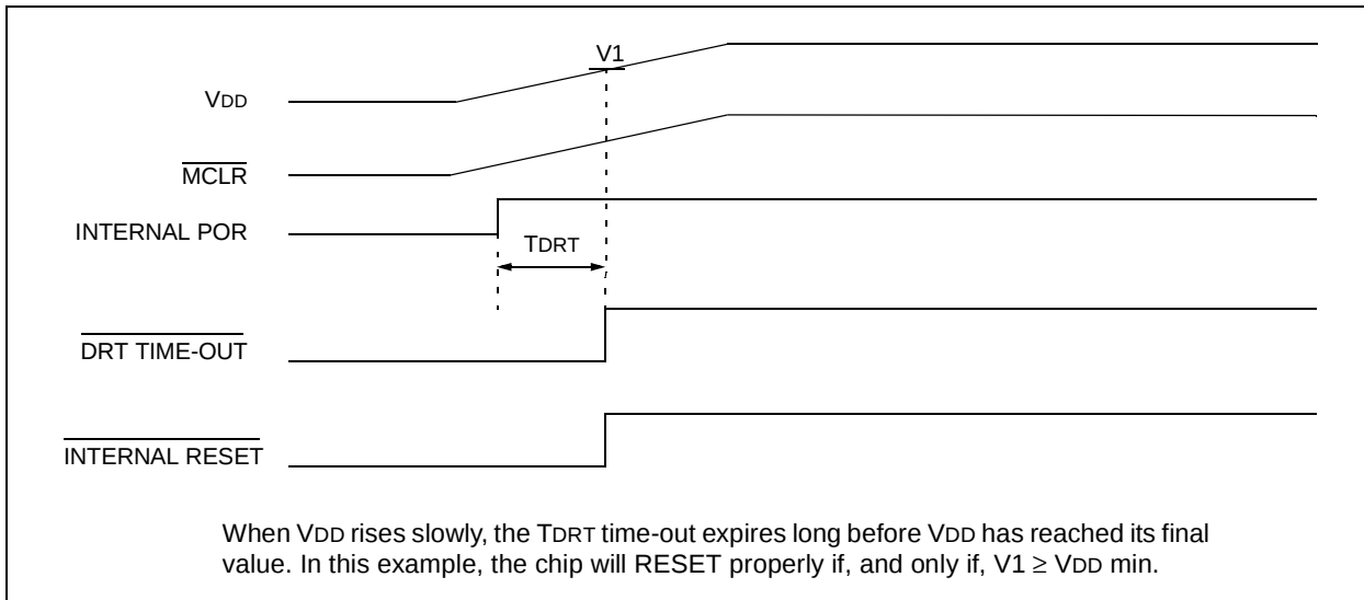
FIGURE 8-9: TIME-OUT SEQUENCE ON POWER-UP ( \overline{\text{MCLR}} TIED TO V_{DD} ): SLOW V_{DD} RISE TIME
