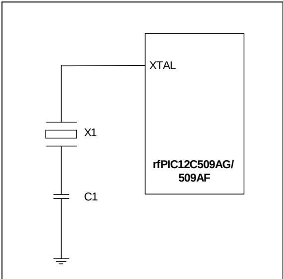
FIGURE 7-2: EXAMPLE ASK EXTERNAL CRYSTAL CIRCUIT
