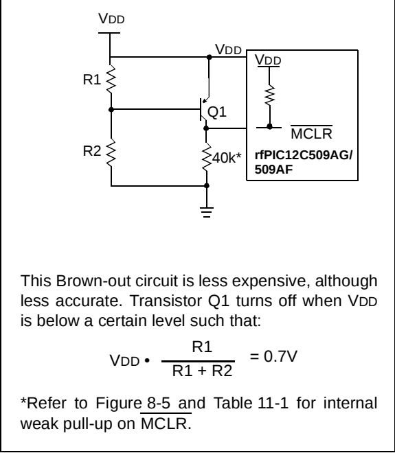
FIGURE 8-13: BROWN-OUT PROTECTION CIRCUIT 3
