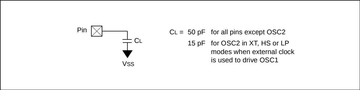
FIGURE 11-3: LOAD CONDITIONS
