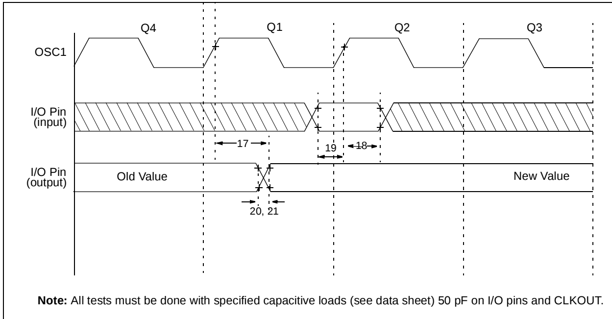
FIGURE 11-5: I/O TIMING
