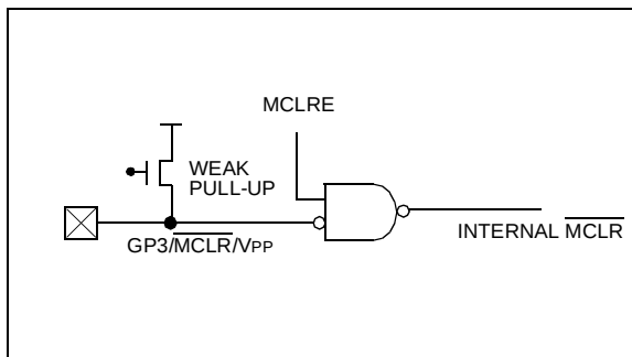
FIGURE 8-5: MCLR SELECT
