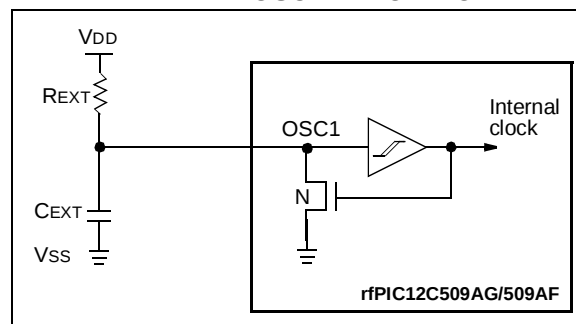
FIGURE 8-4: EXTERNAL RC OSCILLATOR MODE
