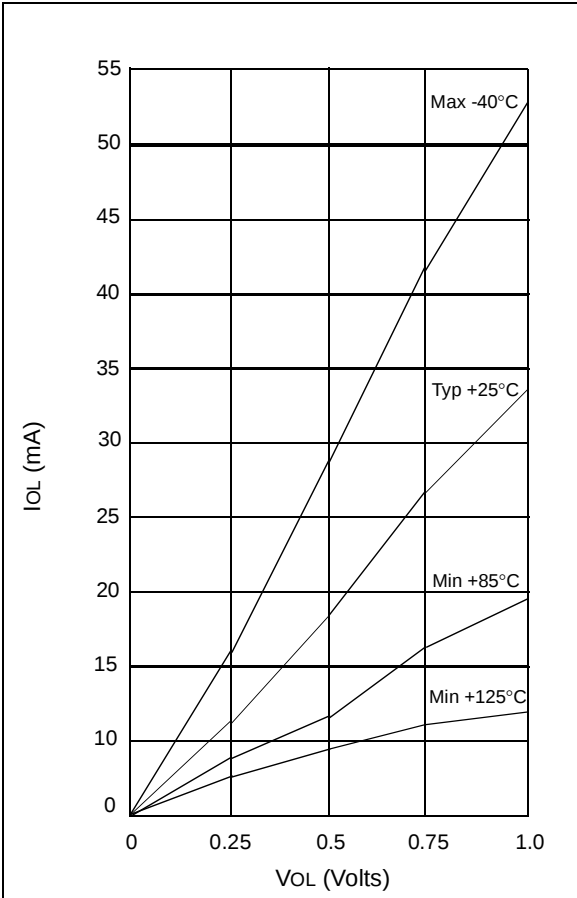
FIGURE 12-12: I_{OL} vs. V_{OL} , V_{DD} = 5.5\text{ V}
