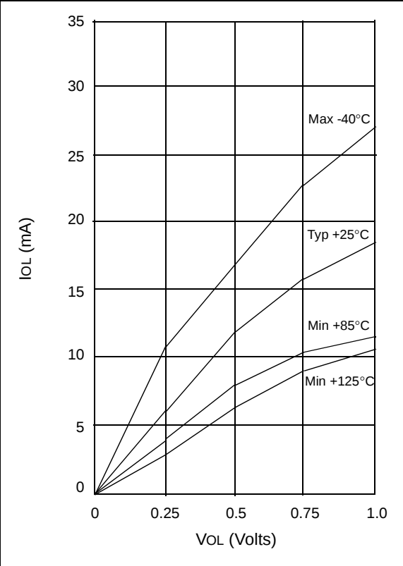
FIGURE 12-10: I_{OL} vs. V_{OL} , V_{DD} = 3.5\text{ V}
