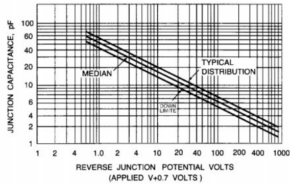
Fig. 2 - JUNCTION CAPACITANCE
