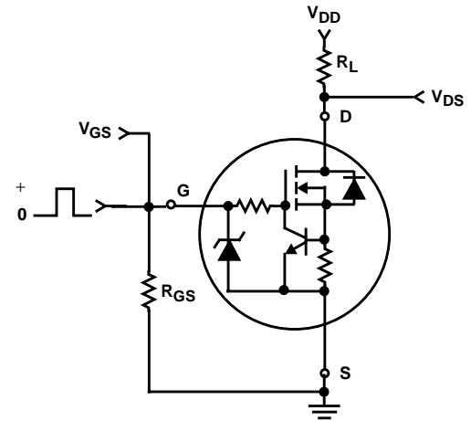
FIGURE 10. SWITCHING TEST CIRCUIT
