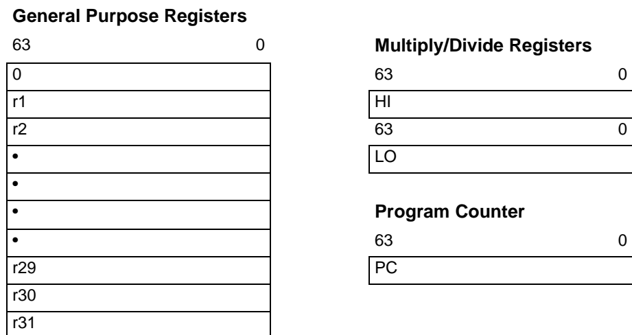
Figure 2 CPU Registers
