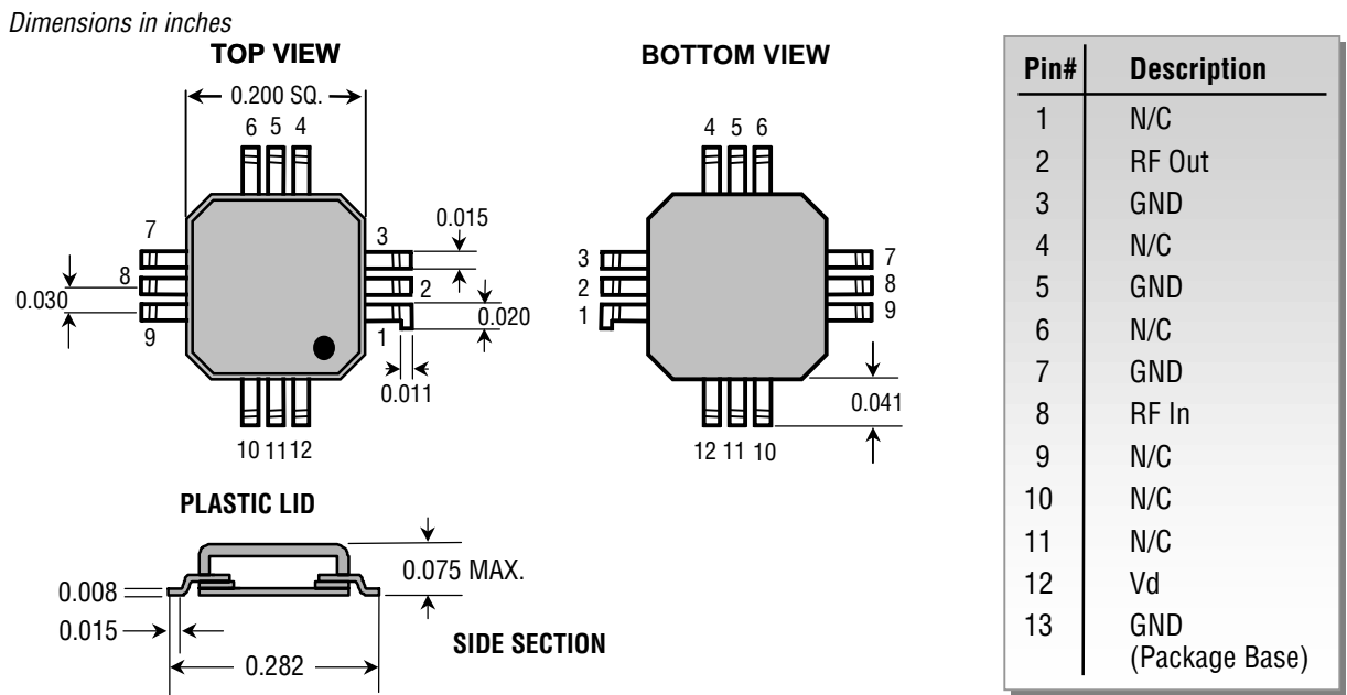
Figure 1 Package Outline and Pin Designations
