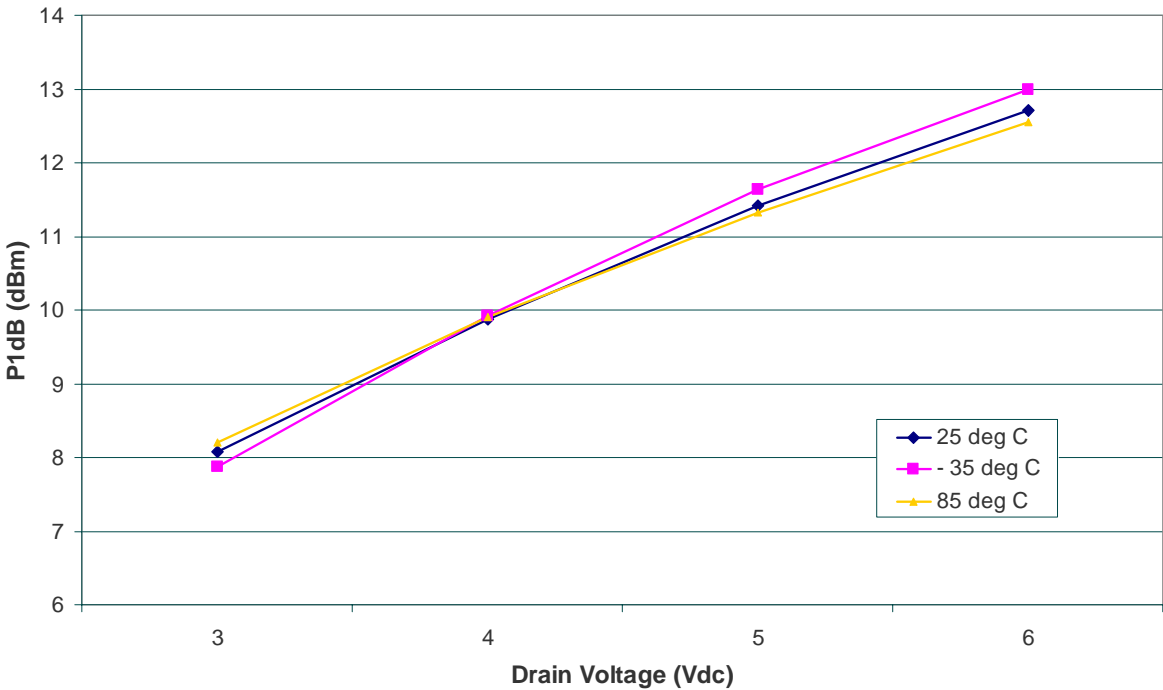
RMLA3565-58 1 dB Compression (5.5 GHz) Vs Drain Voltage and Temperature
