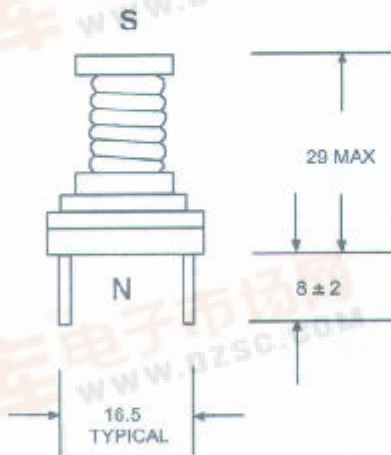
LINEARITY COIL
