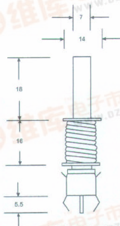
WIDTH COIL
