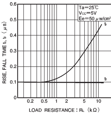
Fig.7 Rise and fall time vs. load resistance
