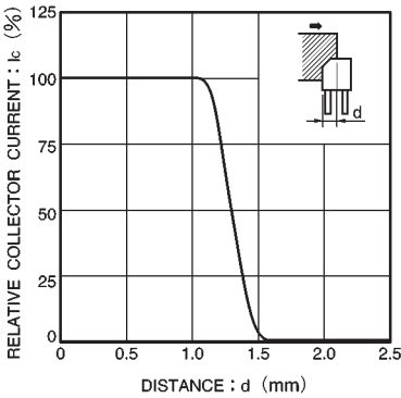
Fig.6 Relative output vs. distance (I)
