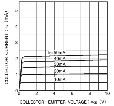
Fig.9 Output characteristics
