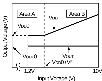
FIG. B Output Voltage vs. Input Voltage characteristic
