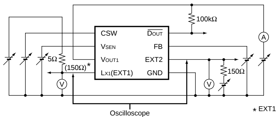
Fig.2 Test Circuit 2
