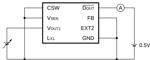
Fig.3 Test Circuit 3
