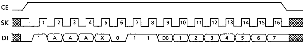
Figure 11 Write mode timing(S-24H30, S-24S30)
