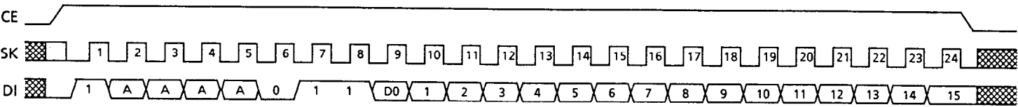
Figure 10 Write mode timing(S-24H45, S-24S45)
