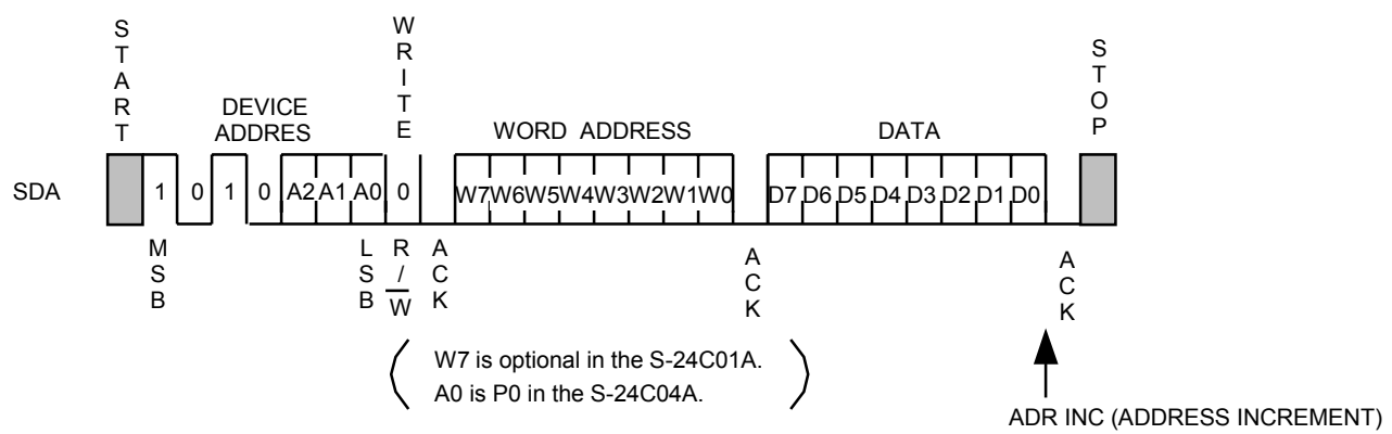
Figure 10 Byte Write
