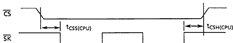
Figure 4 Timing chart of t_{CSS(\text{CPU})} and t_{CSH(\text{CPU})} when connected to CPU
