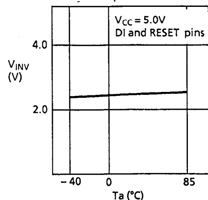
1.23 Input reversal voltage V_{INV} – Ambient temperature T_a
