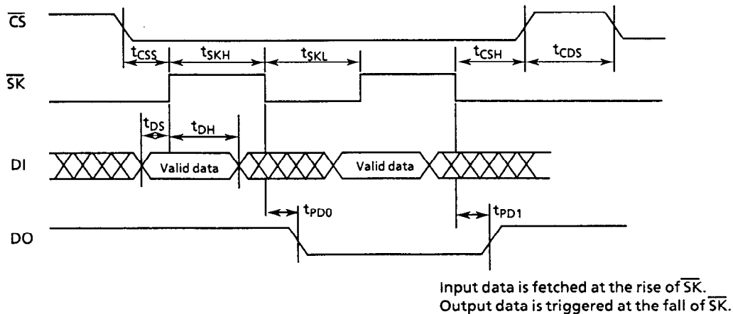
Figure 3 Timing chart
