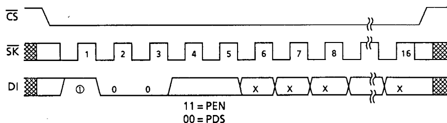
Figure 7 PEN/PDS Timing
