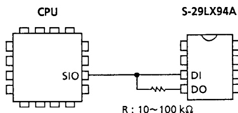
Figure 8 3-wire interface
