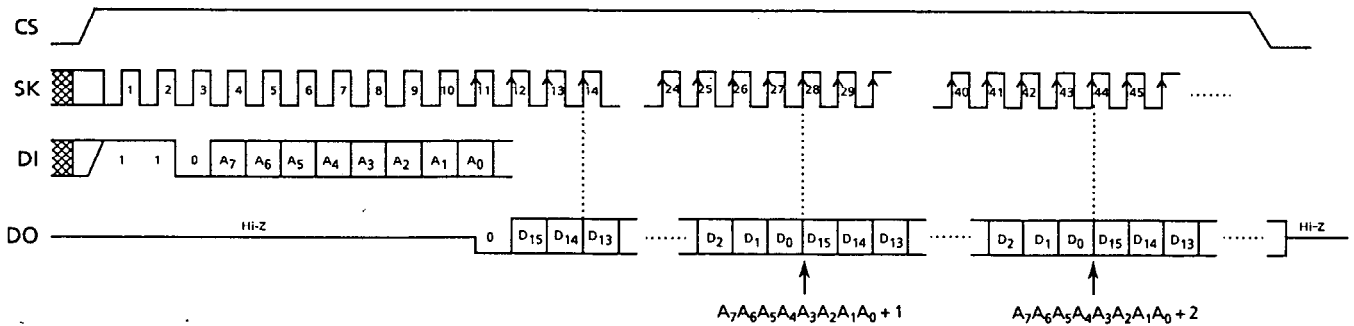
Figure 6 Read Timing (S-29L331A)
