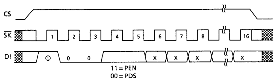
Figure 9 PEN/PDS Timing
