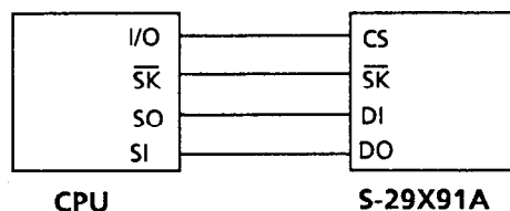
Figure 11 Connectin Example
