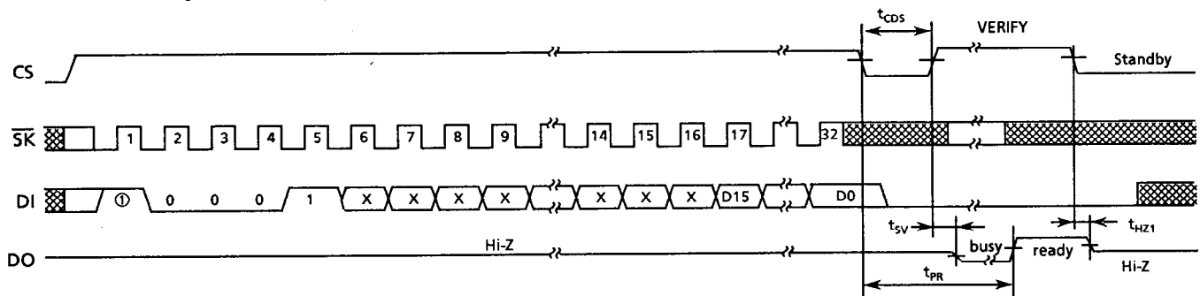
Figure 7 WRAL Timing
