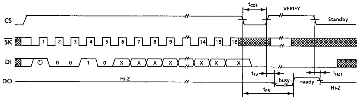
Figure 8 ERAL Timing
