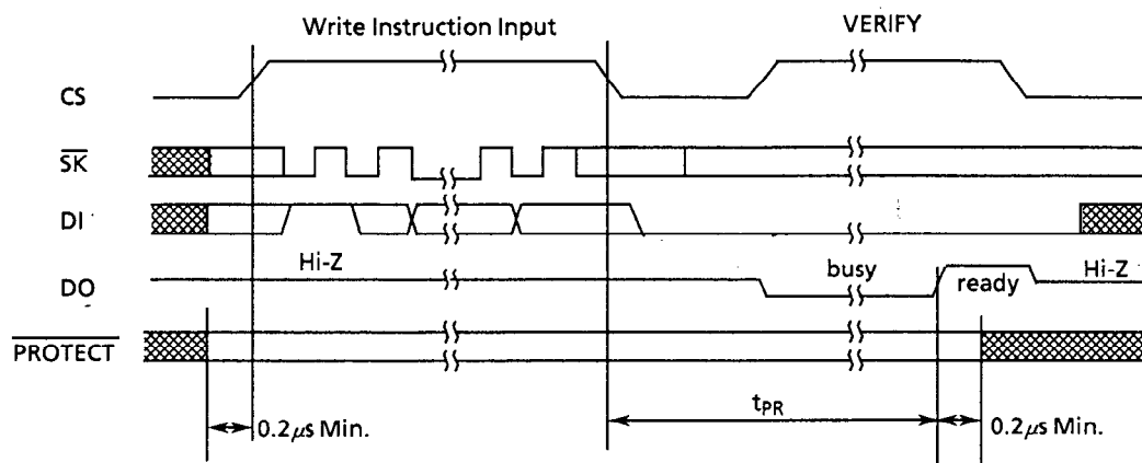
Figure 13 \overline{\text{PROTECT}} Terminal Input Signal Timing
