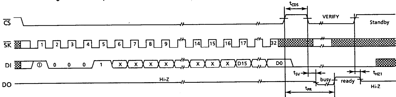
Figure 7 WRAL Timing
