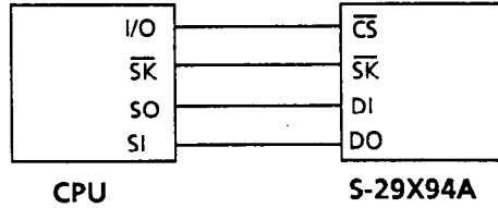
Figure 11 Connectin Example
