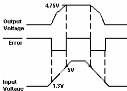
Figure 1. Error Output Timing
