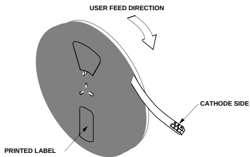
Figure 8. Reeling Orientation.
