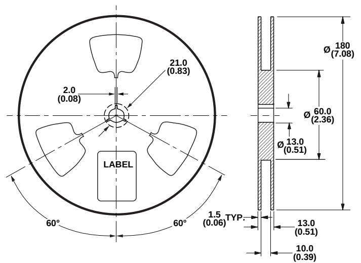
Figure 9. Reel Dimensions.
