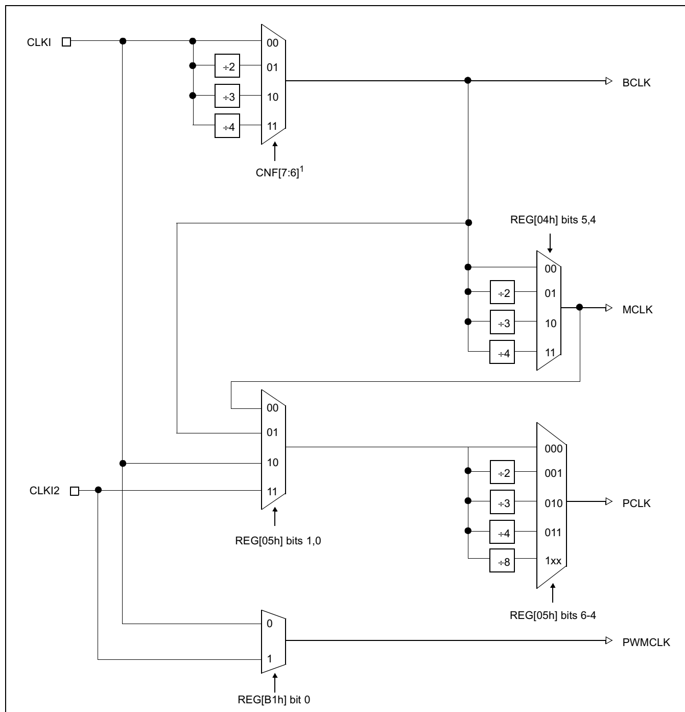
Figure 7-1: Clock Selection
