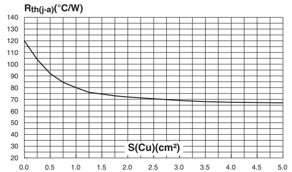
Figure 12: Thermal resistance junction to ambient versus copper surface under each lead (Epoxy printed circuit board FR4, copper thickness: 35 \mu\text{m} ) (SMA)
