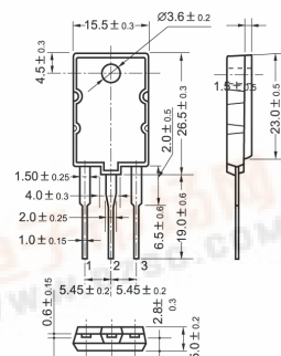
TO-3PH
