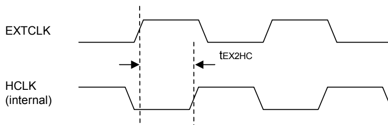
Figure 25-4. EXTCLK/HCLK in case that EXTCLK is used without the PLL
