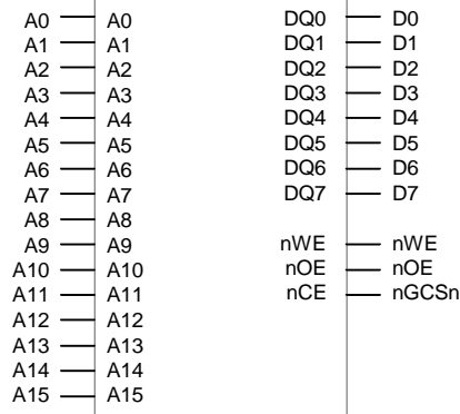
Figure 5-4. Memory Interface with 8-bit ROM
