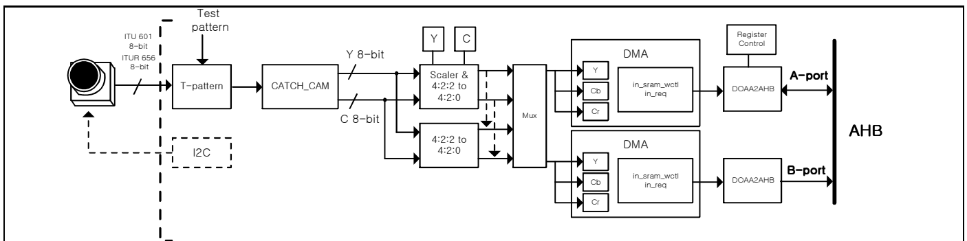
Figure 23-1. Camera interface overview
