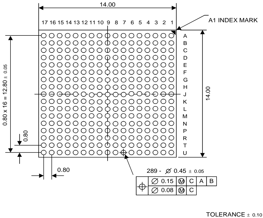
Figure 26-2. 289-FBGA-1414 Package Dimension 2 (Bottom View)
