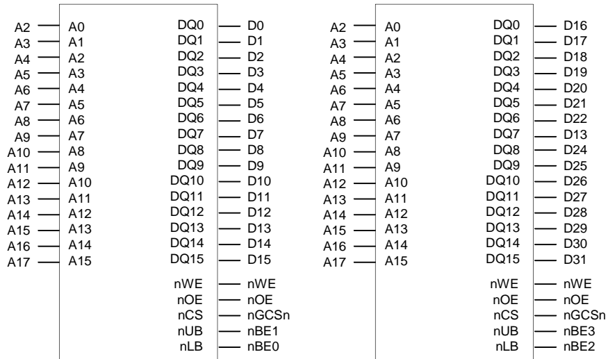
Figure 5-9. Memory Interface with 16-bit SRAM x 2
