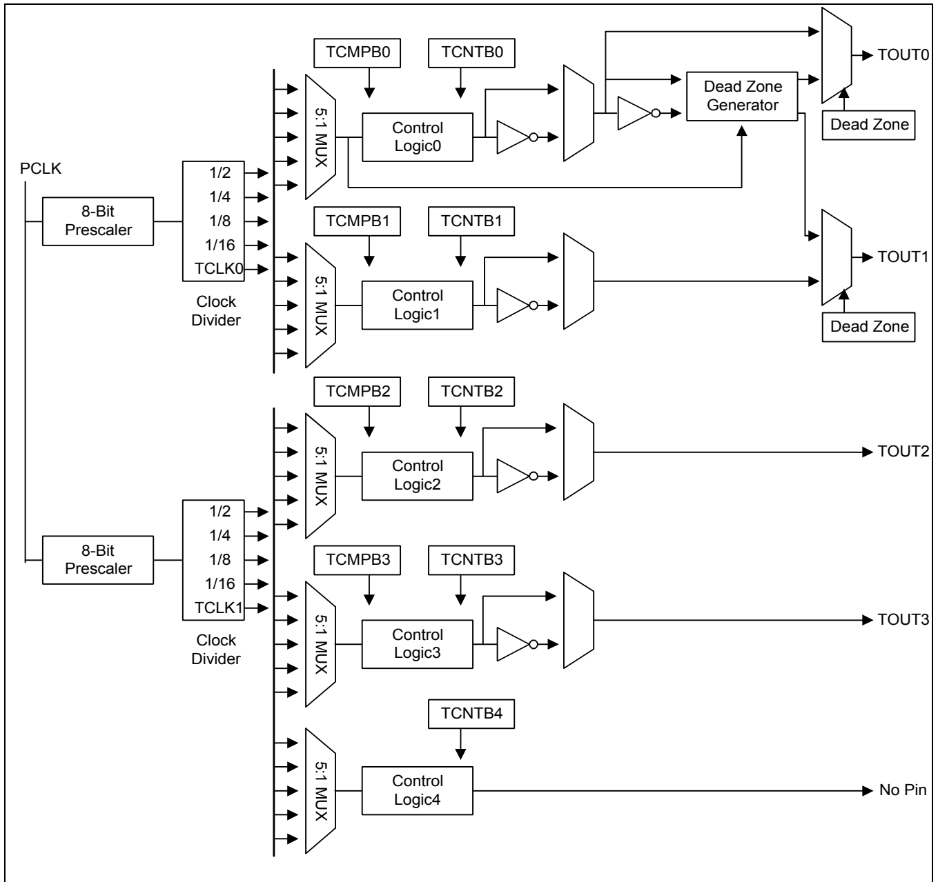
Figure 10-1. 16-bit PWM Timer Block Diagram
