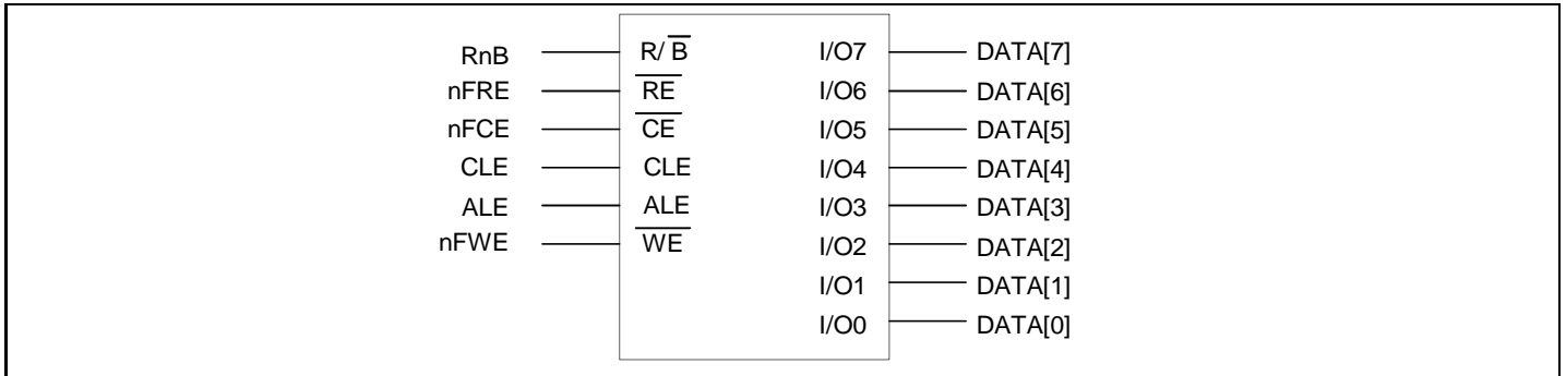
Figure 6-1 A 8-bit NAND Flash Memory Interface
