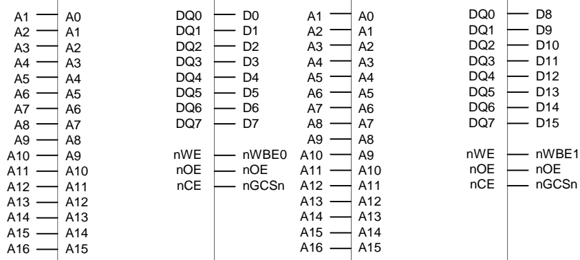
Figure 5-5. Memory Interface with 8-bit ROM x 2
