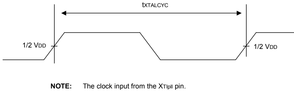
Figure 25-2. XTlpII Clock Timing
