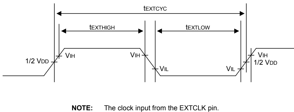
Figure 25-3. EXTCLK Clock Input Timing
