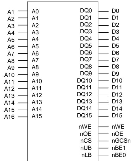
Figure 5-8. Memory Interface with 16-bit SRAM
