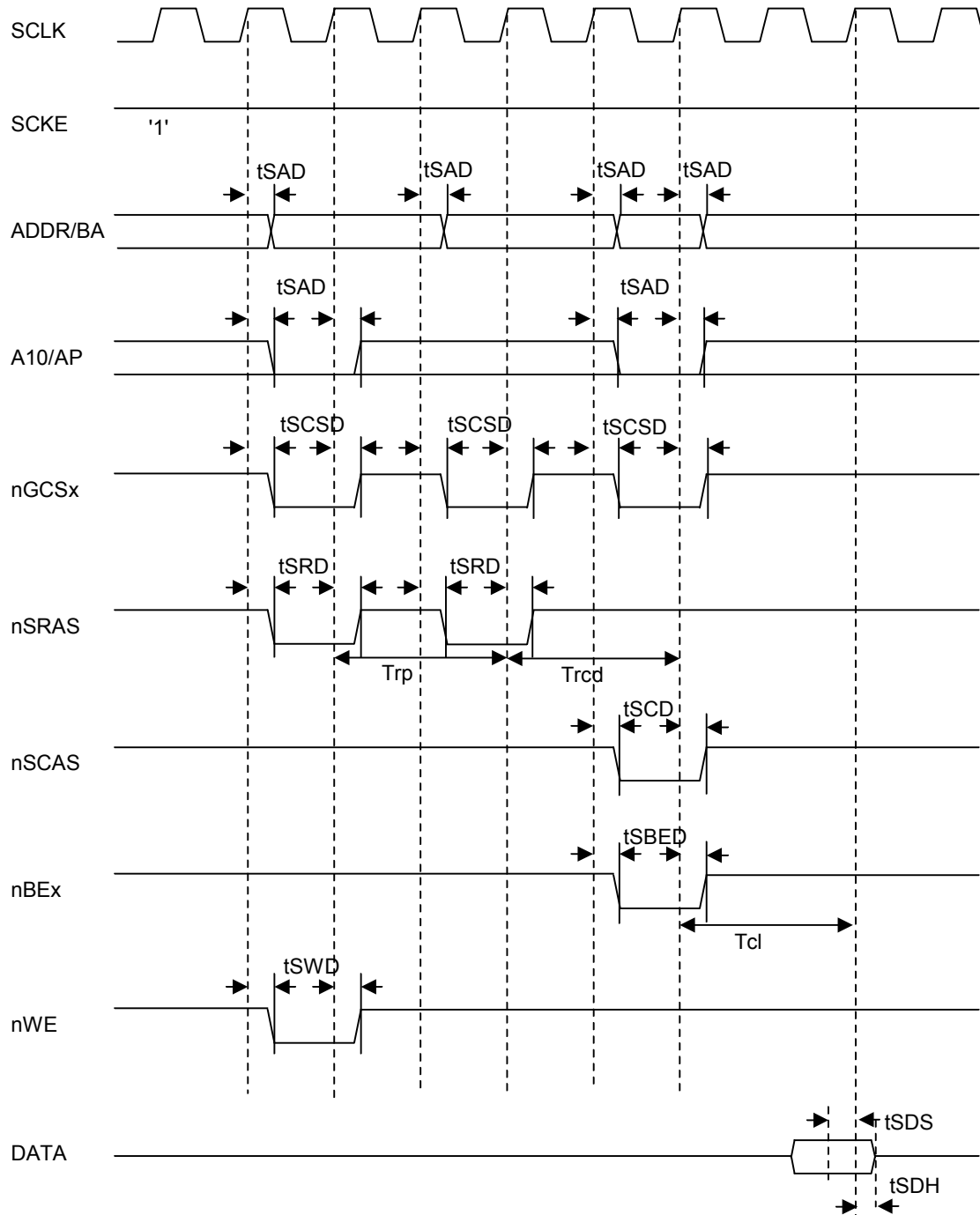
Figure 25-23. SDRAM Single READ Timing(I) ( Trp=2 , Trcd=2 , Tcl=2 )
