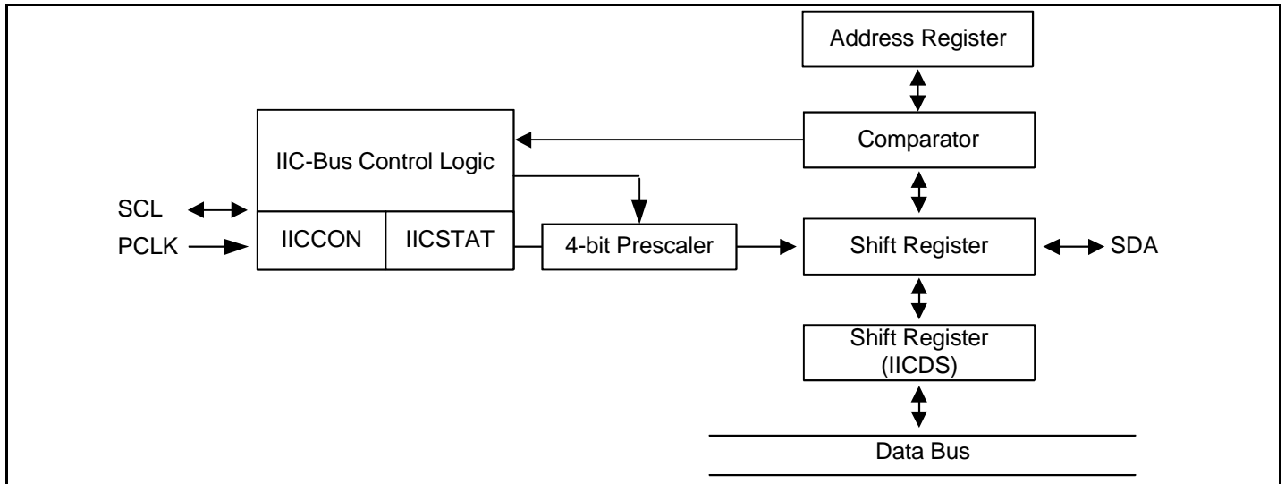
Figure 20-1. IIC-Bus Block Diagram
