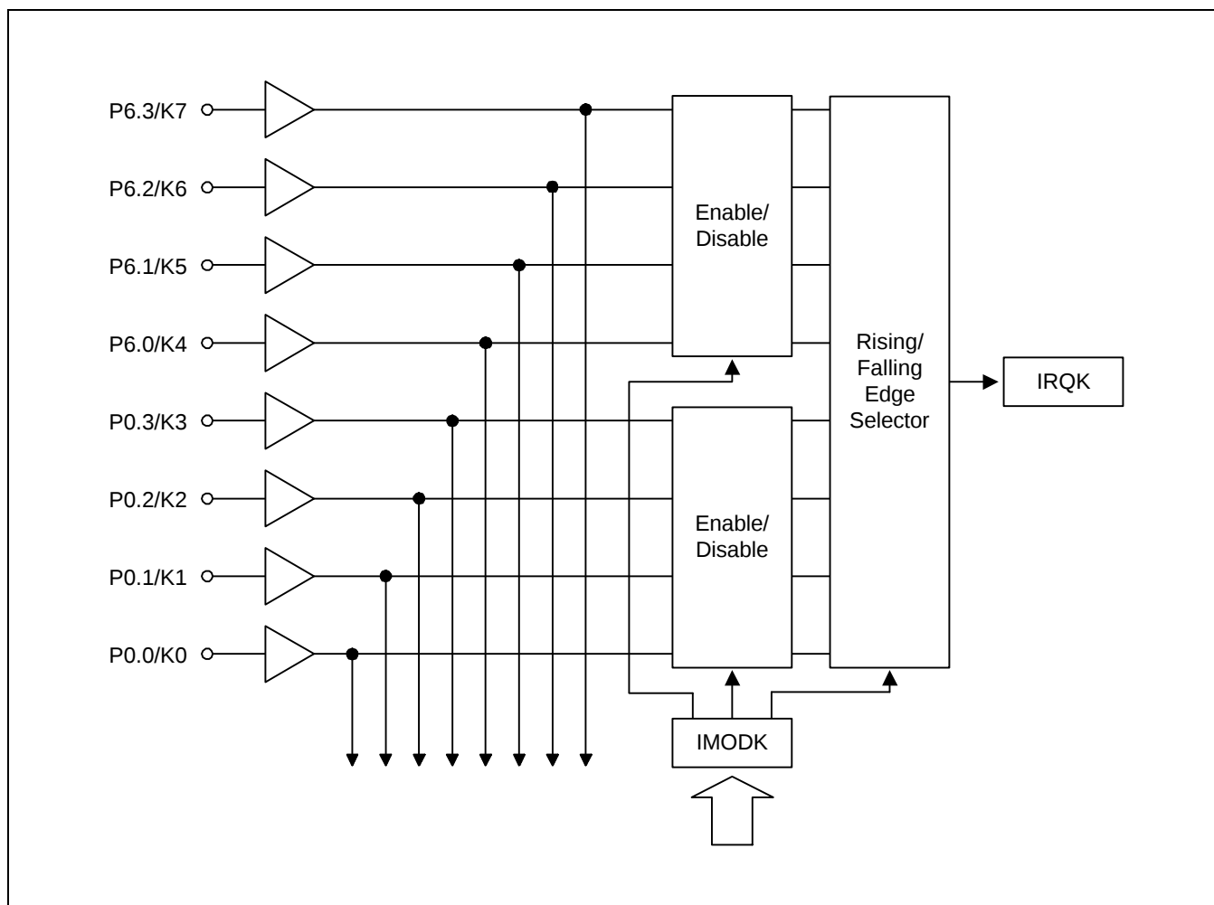
Figure 7-6. Circuit Diagram for INTK
