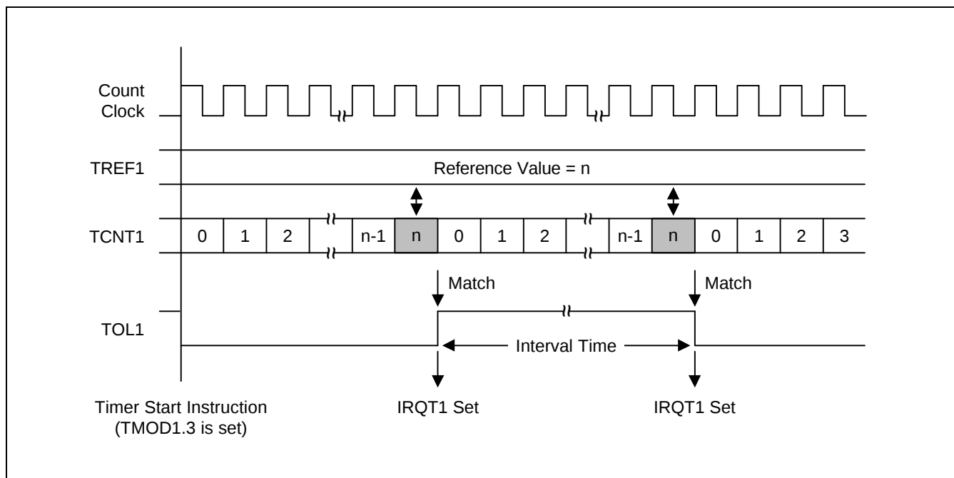
Figure 11-5. TC1 Timing Diagram
