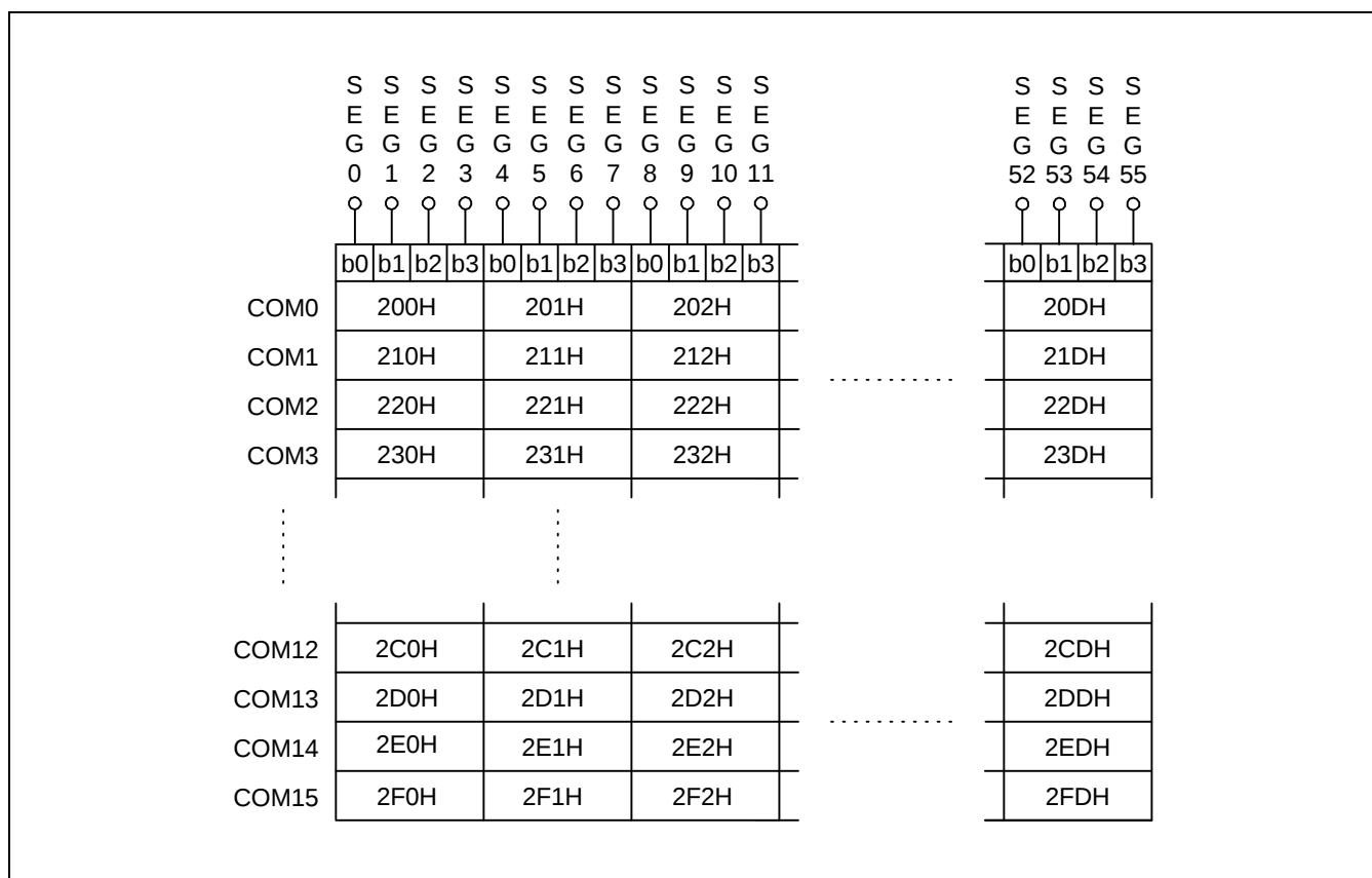
Figure 12-3. LCD Display Data RAM Organization
