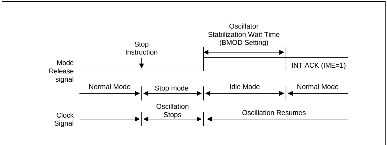
Figure 8-4. Timing When Stop Mode is Released by an Interrupt
