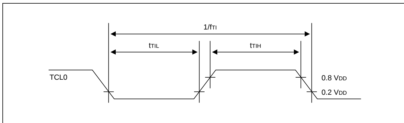
Figure 14-7. TCL Timing
