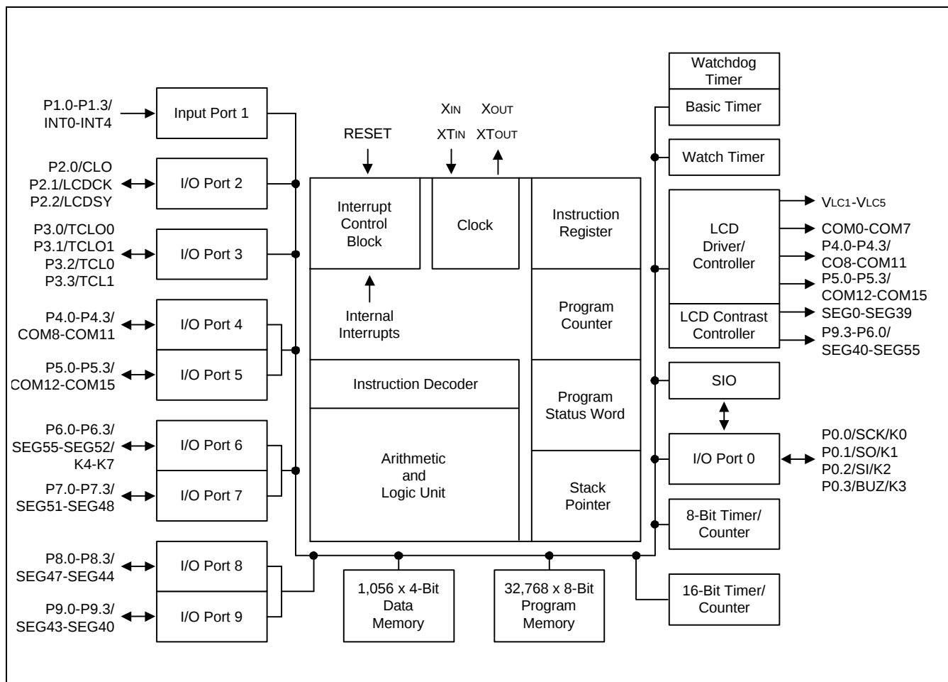
Figure 1-1. S3C72P9/P72P9 Simplified Block Diagram
