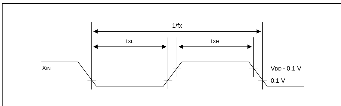
Figure 17-5. Clock Timing Measurement at X_{IN}
