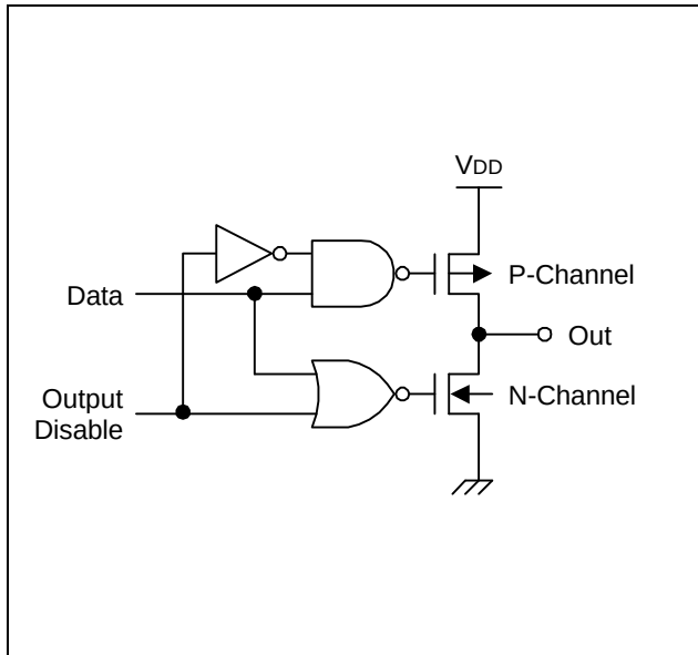
Figure 1-9. Pin Circuit Type C
