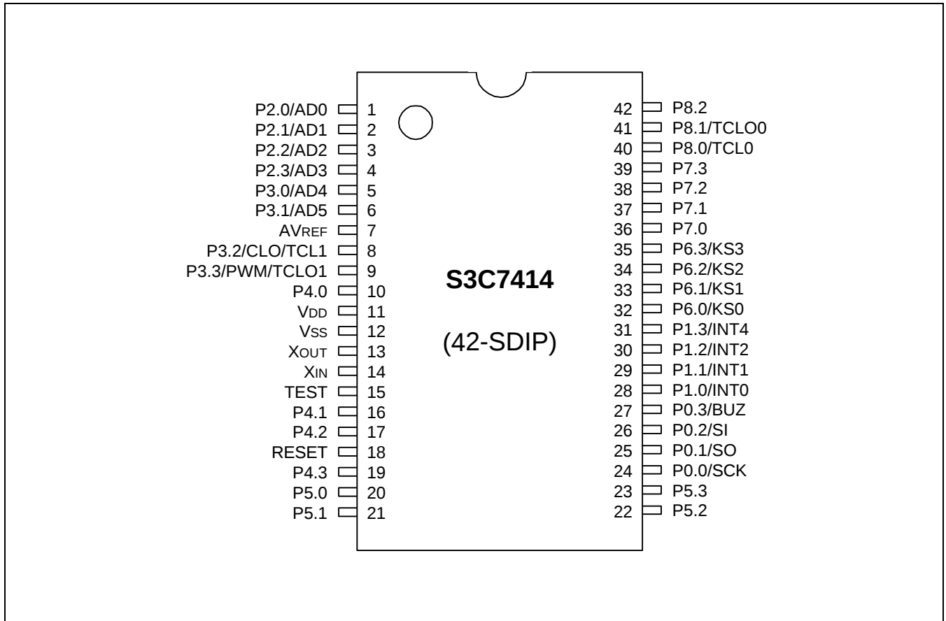
Figure 1-2. S3C7414 Pin Assignment (42-SDIP)
