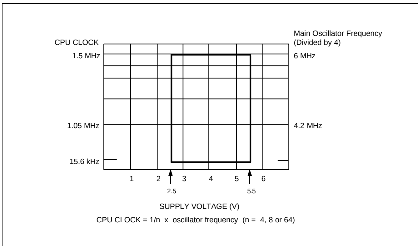
Figure 16-9. S3P7434 Standard Operating Voltage Range
