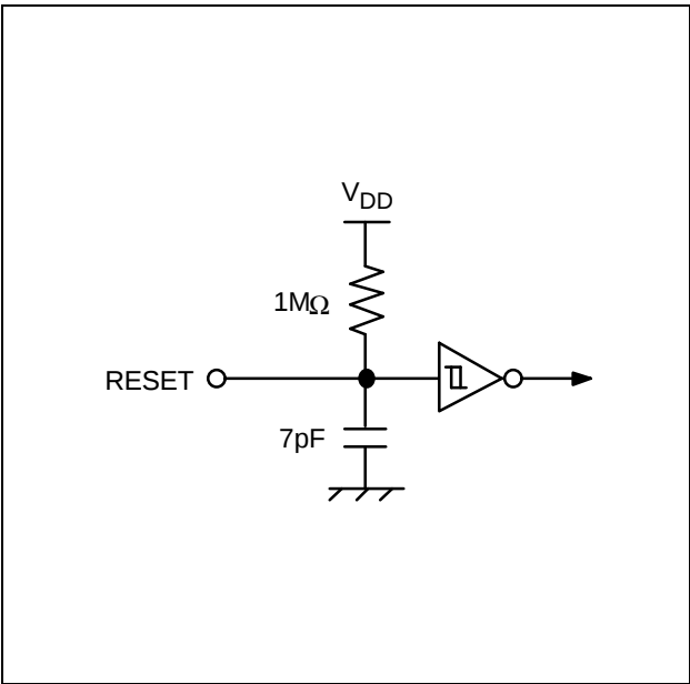
Figure 1-10. Pin Circuit Type B-2
