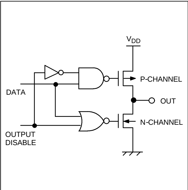
Figure 1-11. Pin Circuit Type C
