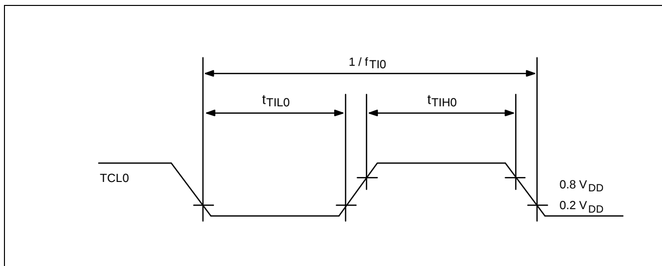
Figure 14-7. TCL0/1 Timing
