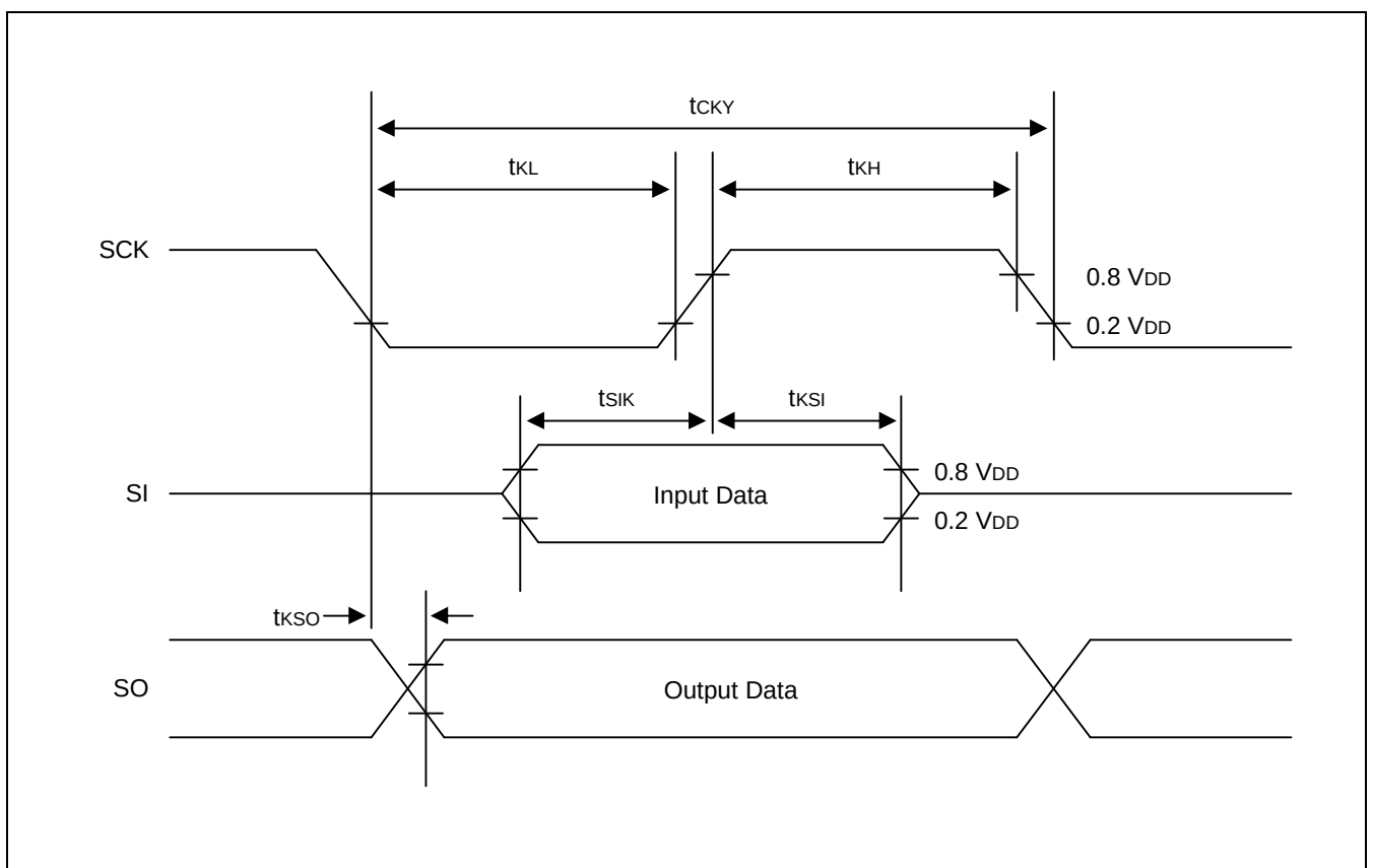
Figure 19-5. Serial Data Transfer Timing
