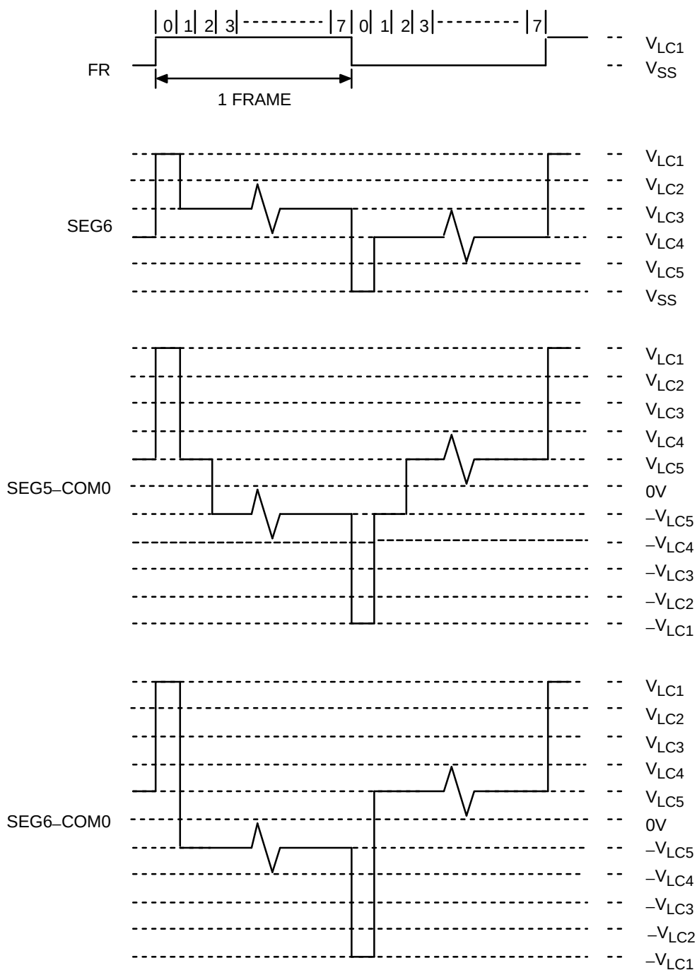
Figure 15-11. LCD Signal Waveforms (1/8 Duty, 1/5 Bias) (Continued)
