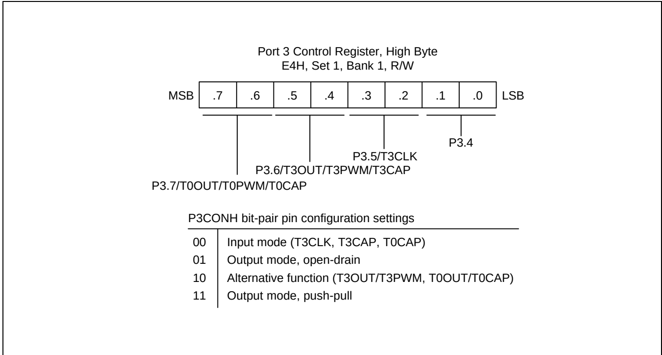
Figure 9-6. Port 3 High-Byte Control Register (P3CONH)
