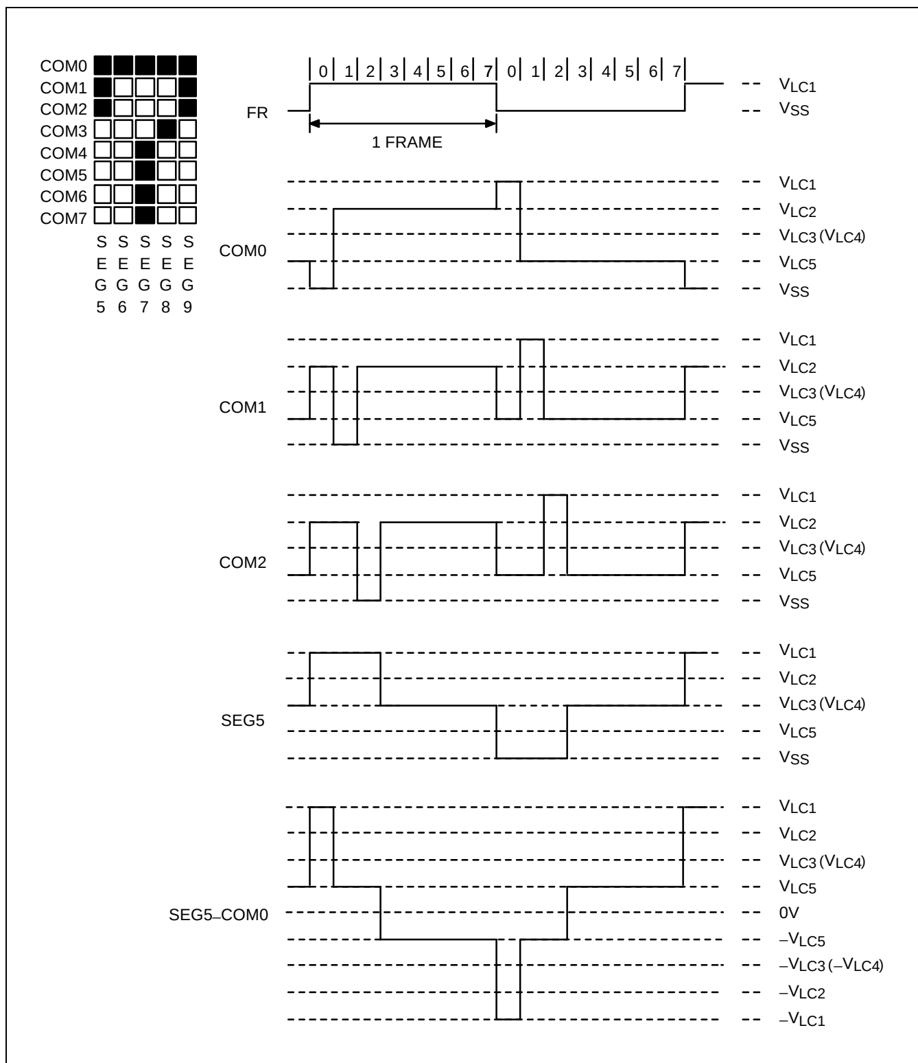
Figure 15-10. LCD Signal Waveforms (1/8 Duty, 1/4 Bias)
