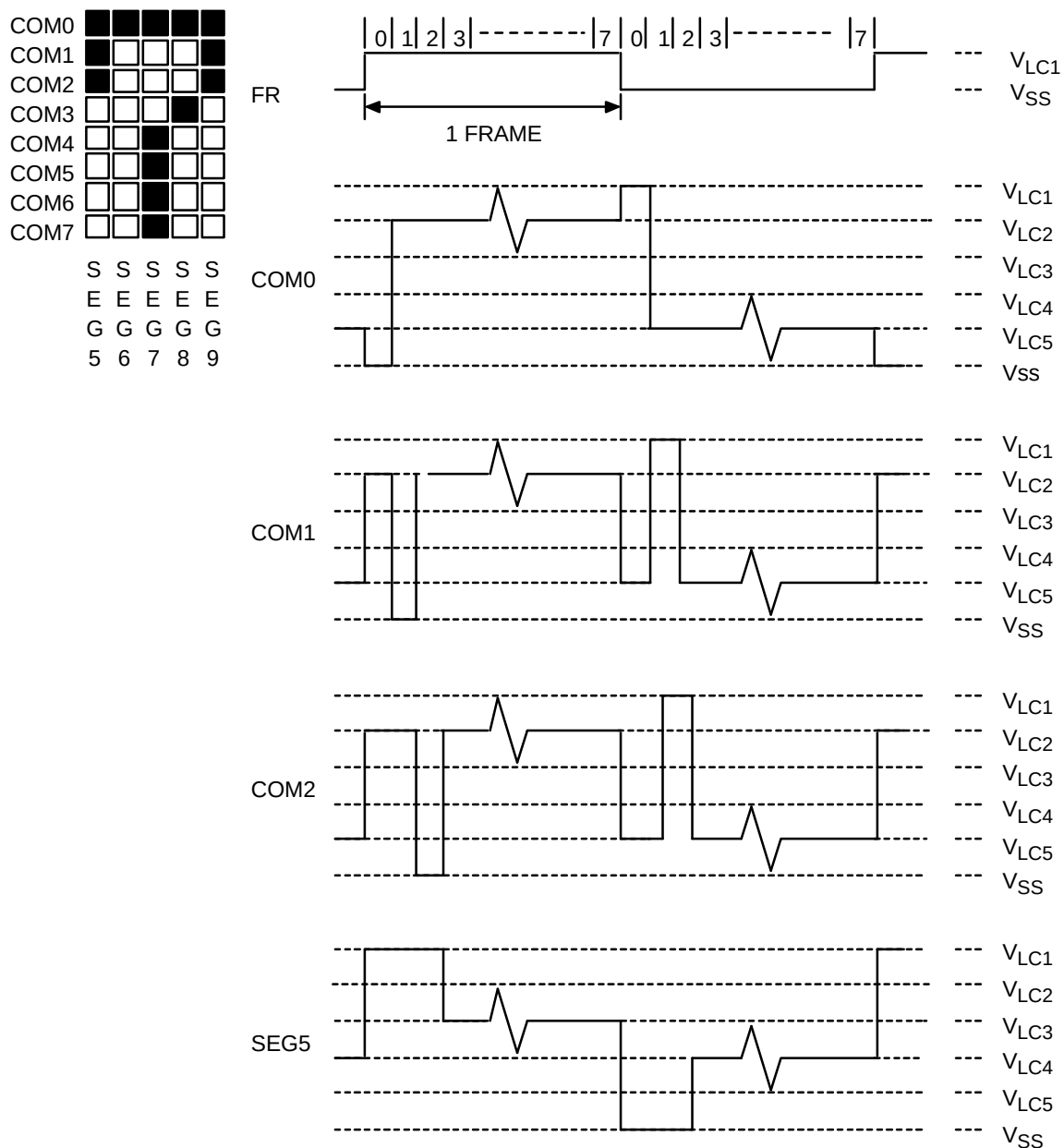
Figure 15-11. LCD Signal Waveforms (1/8 Duty, 1/5 Bias)
