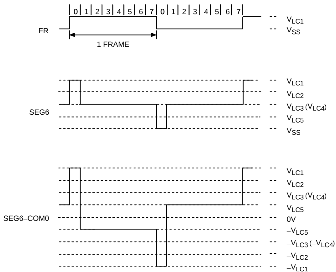
Figure 15-10. LCD Signal Waveforms (1/8 Duty, 1/4 Bias) (Continued)
