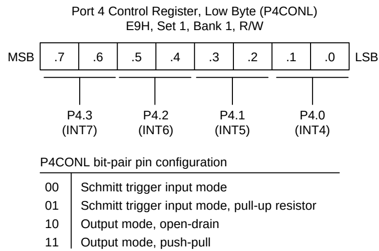
Figure 9-10. Port 4 Low-Byte Control Register (P4CONL)
