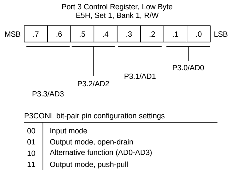
Figure 9-7. Port 3 Low-Byte Control Register (P3CONL)
