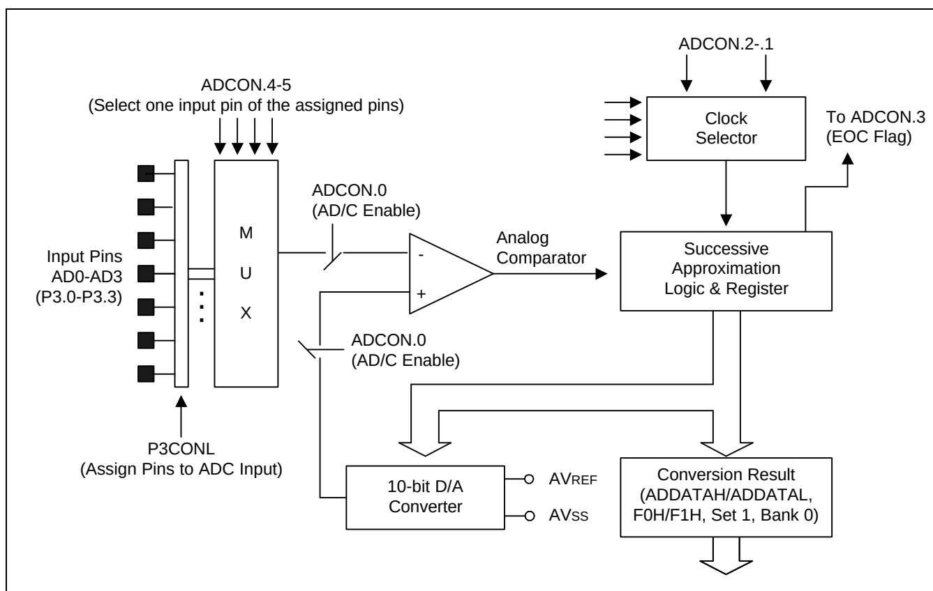
Figure 16-3. A/D Converter Functional Block Diagram
