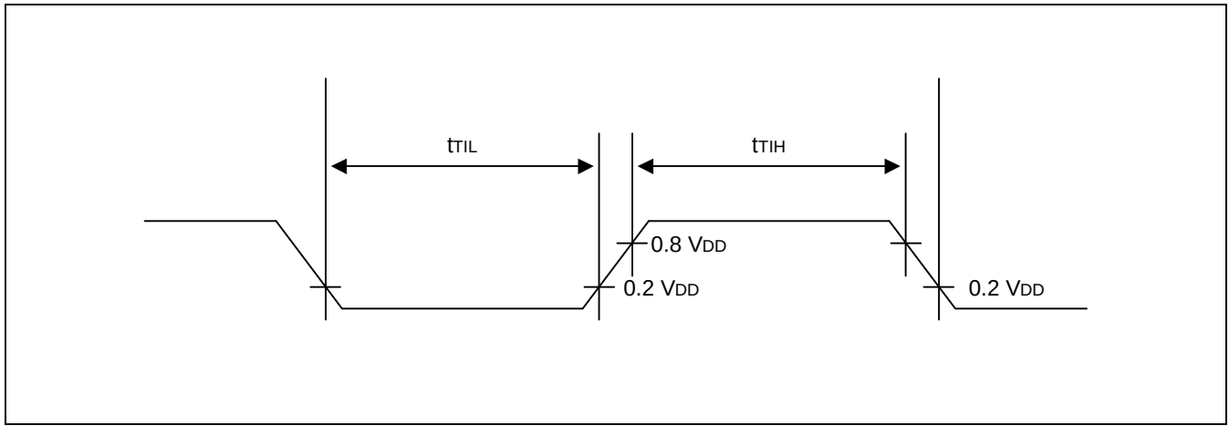
Figure 19-1. Input Timing for External Interrupts (P2.4–P2.7, P4)
