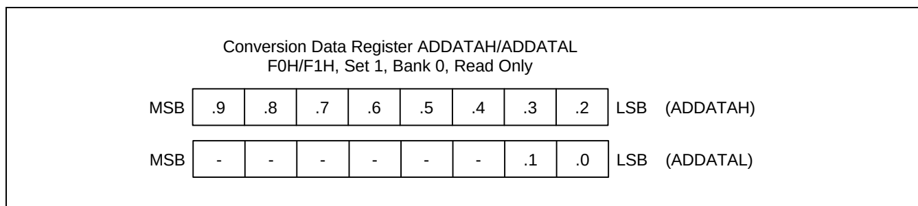
Figure 16-2. A/D Converter Data Register (ADDATAH/ADDATAL)
