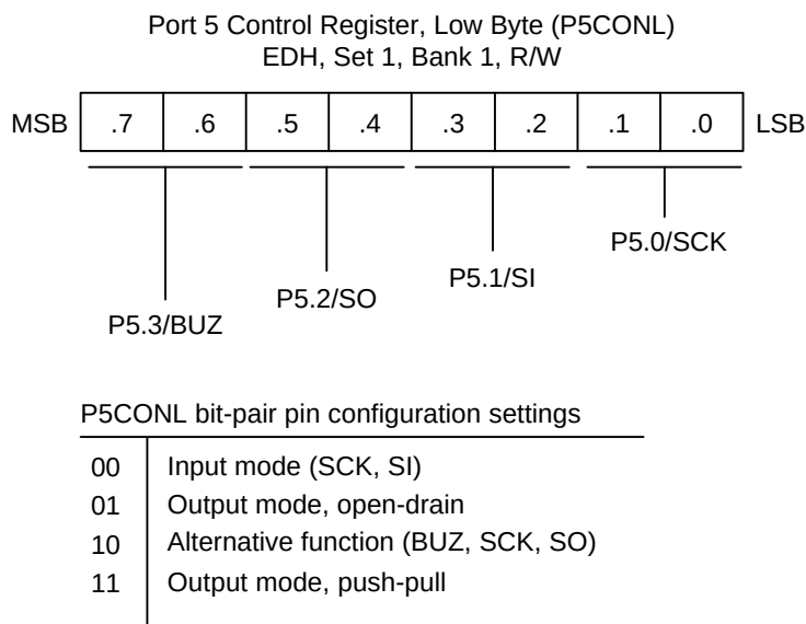
Figure 9-15. Port 5 Low-Byte Control Register (P5CONL)
