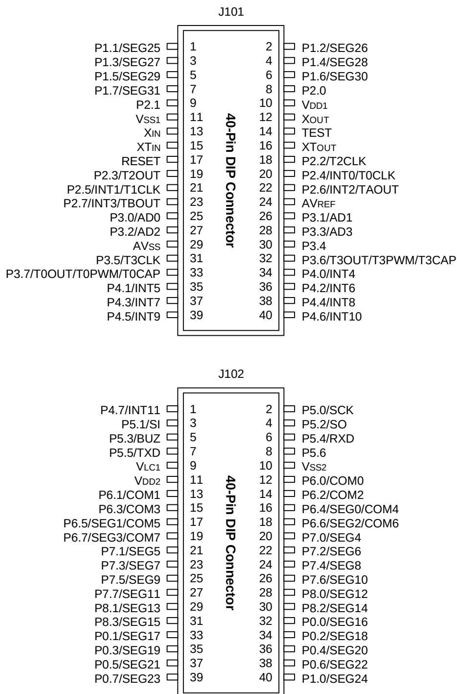
Figure 22-3. 40-Pin Connectors (J101, J102) for TB825A
