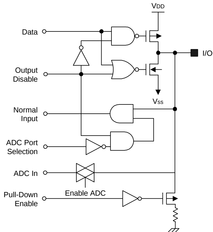
Figure 1-5. Pin Circuit Type 2 (ADC0-ADC3)
