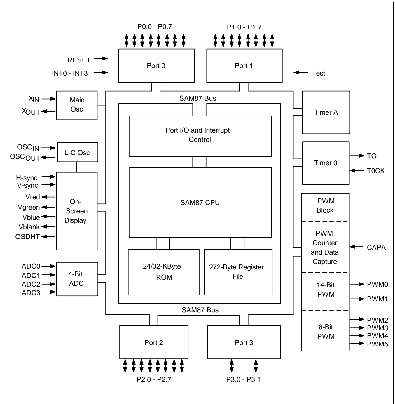
Figure 1-1. Block Diagram
