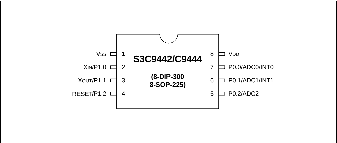
Figure 1-4. Pin Assignment Diagram (8-Pin DIP/SOP Package)
