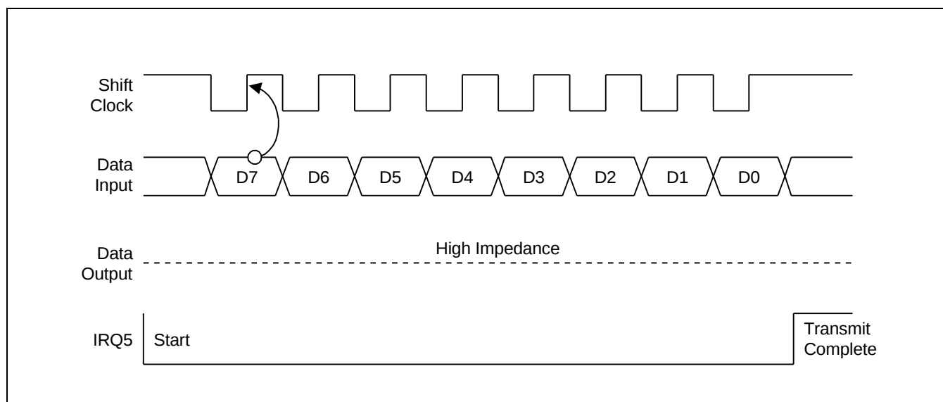
Figure 15-6. Serial I/O Timing in Receive-Only Mode
