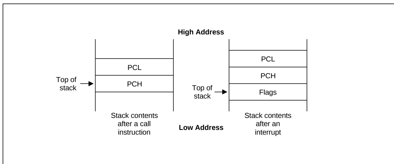
Figure 2-5. Stack Operations
