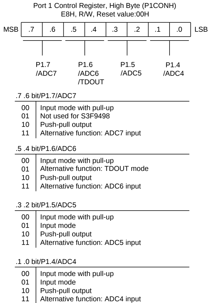
Figure 9-2. Port 1 High-Byte Control Register (P1CONH)
