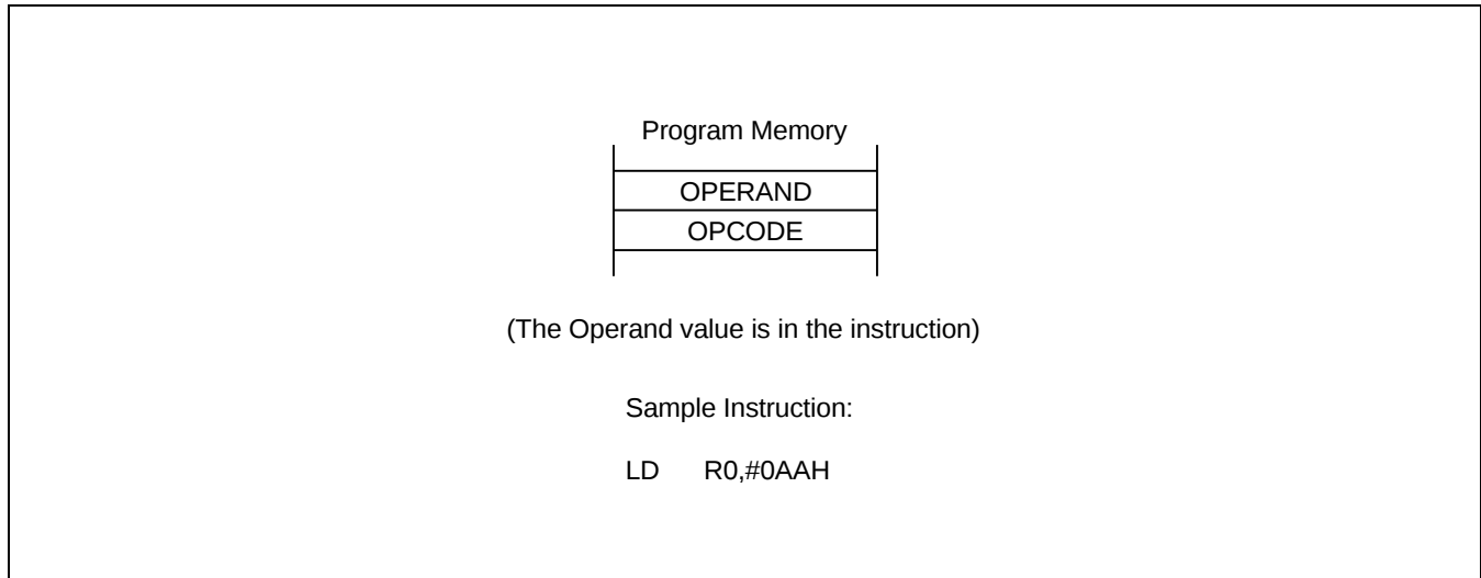
Figure 3-13. Immediate Addressing
