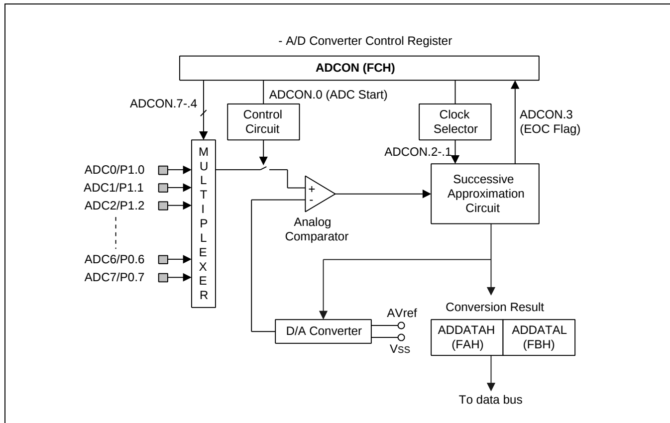
Figure 17-3. A/D Converter Functional Block Diagram
