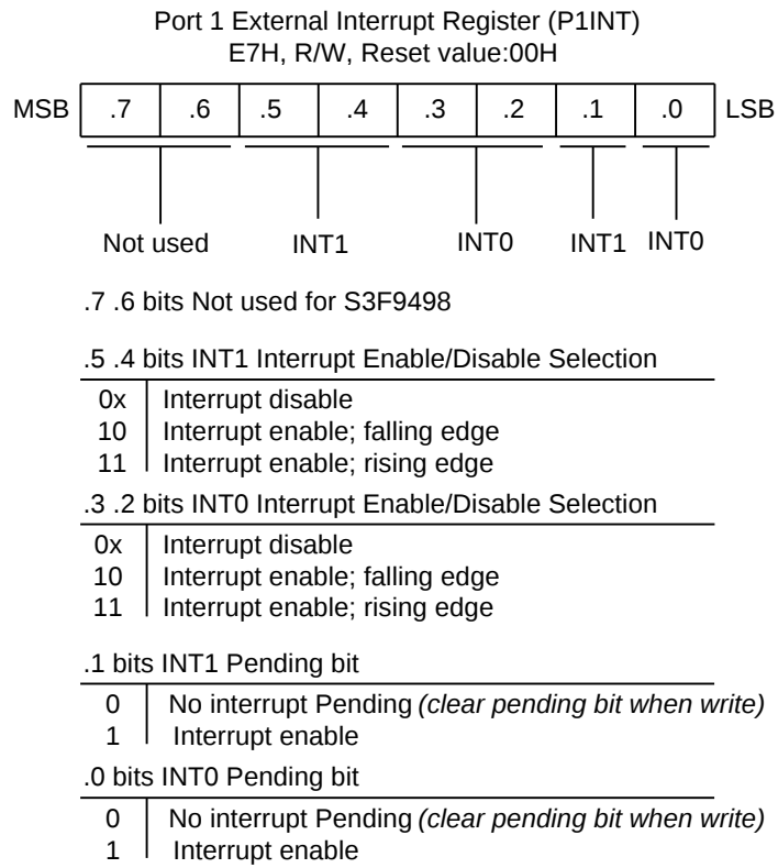
Figure 9-4. Port 1 Interrupt Control Register P1PND)
