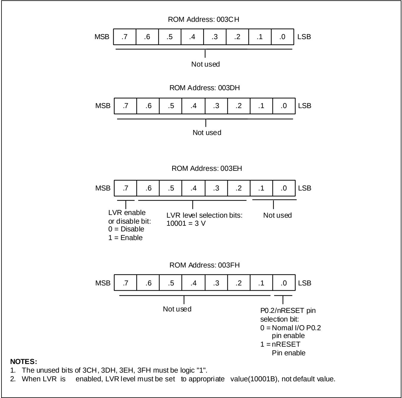
Figure 2-2. Smart Option
