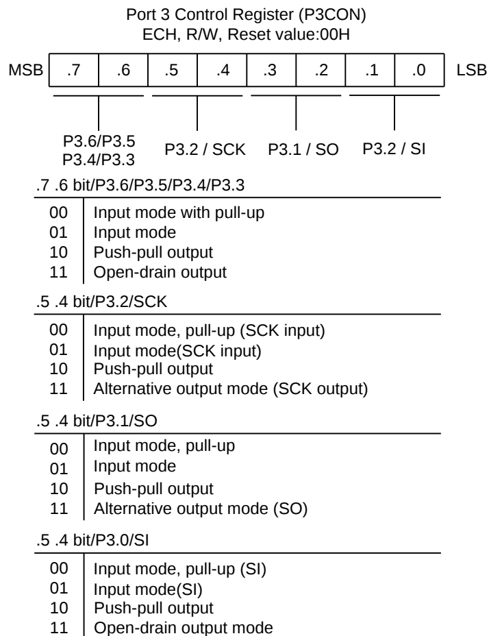
Figure 9-7. Port 3 High-Byte Control Register (P3CON)
