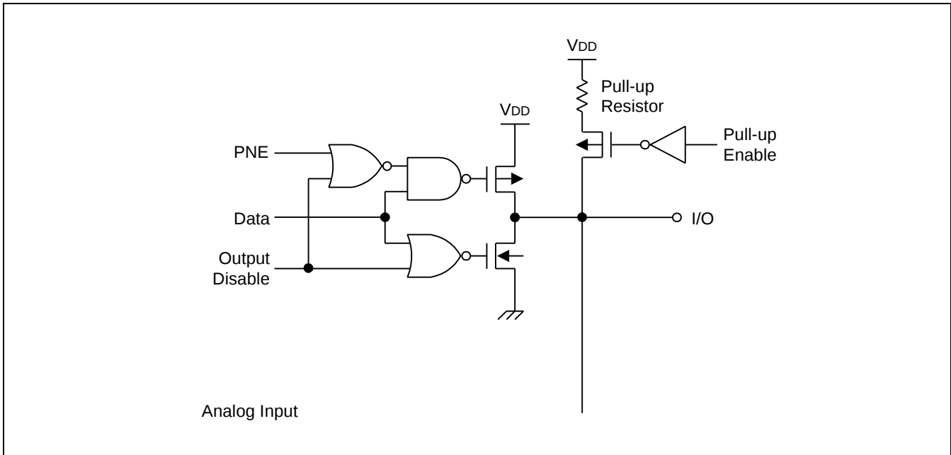
Figure 1-9. Pin Circuit Type E-1
