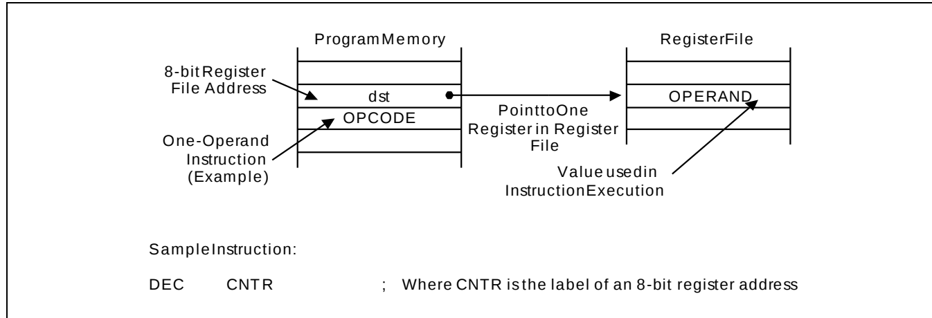
Figure 3-1. Register Addressing
