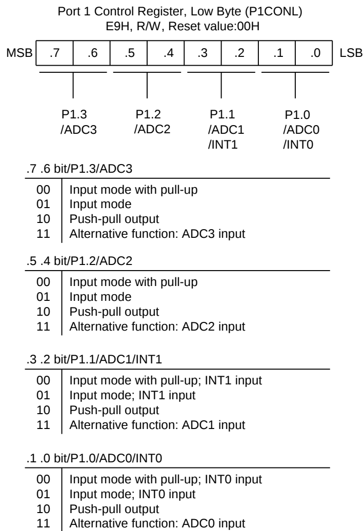
Figure 9-3. Port 1 Low-Byte Control Register (P1CONL)
