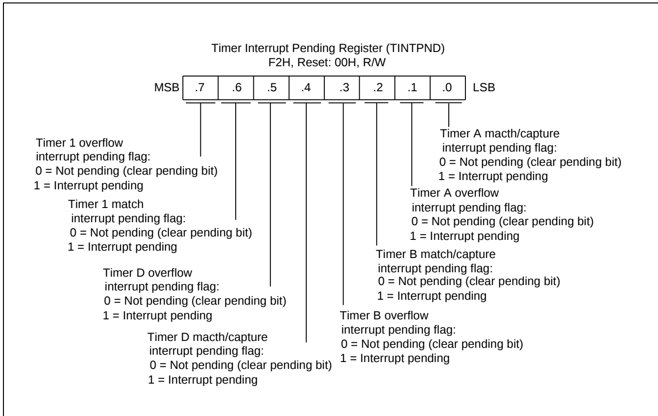
Figure 12-2. Timer A/B/D and TIMER 1 Pending Register (TINTPND)
