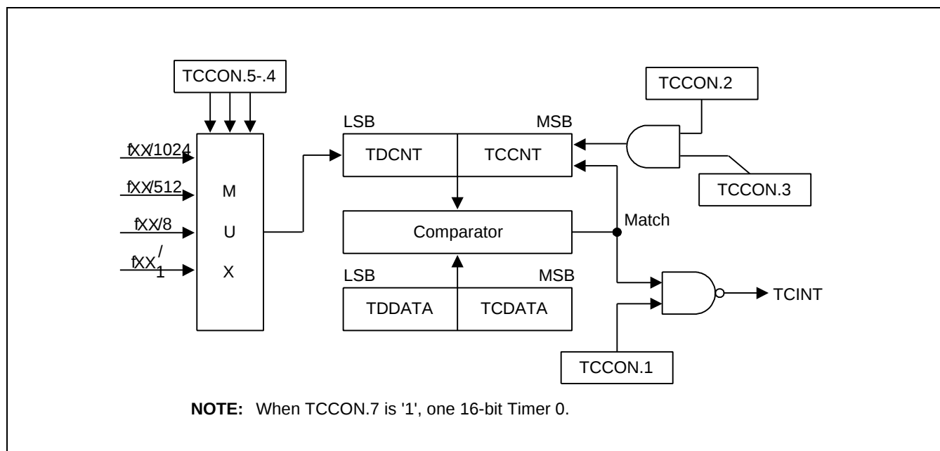
Figure 13-2. Timer 0 Functional Block Diagram
