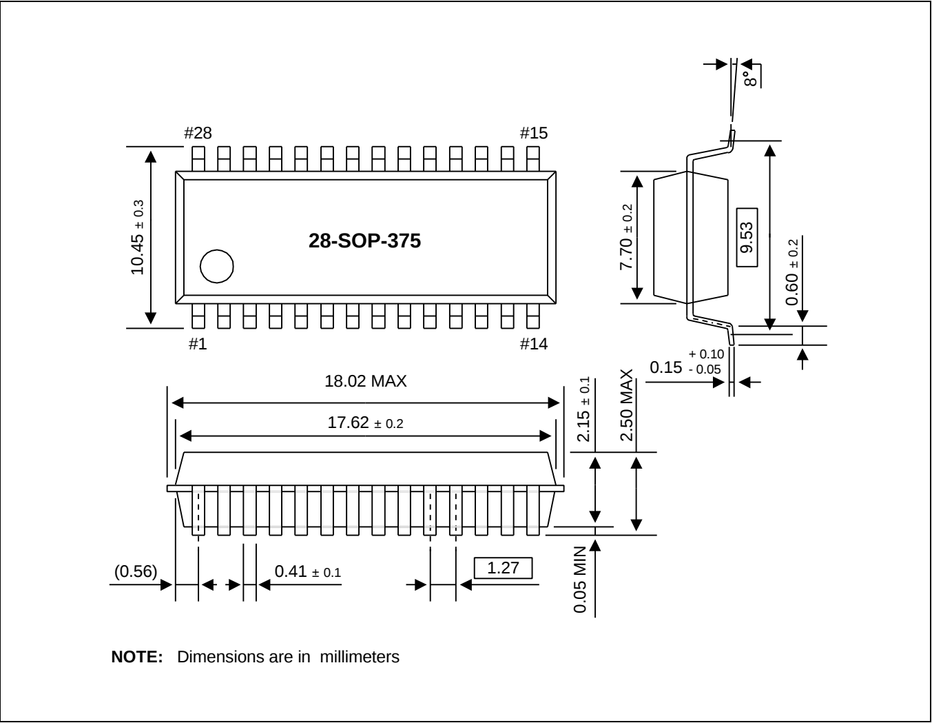
Figure 19-3. 28-SOP-375 Package Dimensions
