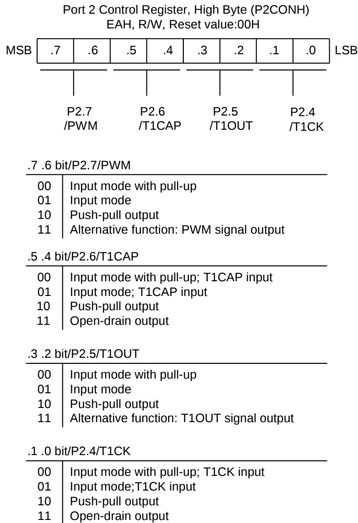
Figure 9-5. Port 2 High-Byte Control Register (P2CONH)
