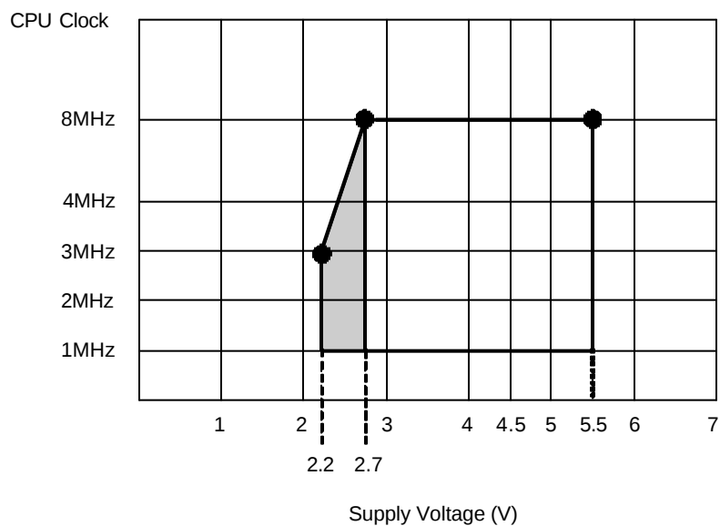
Figure 18-2. Operating Voltage Range (S3C9498/F9498)
