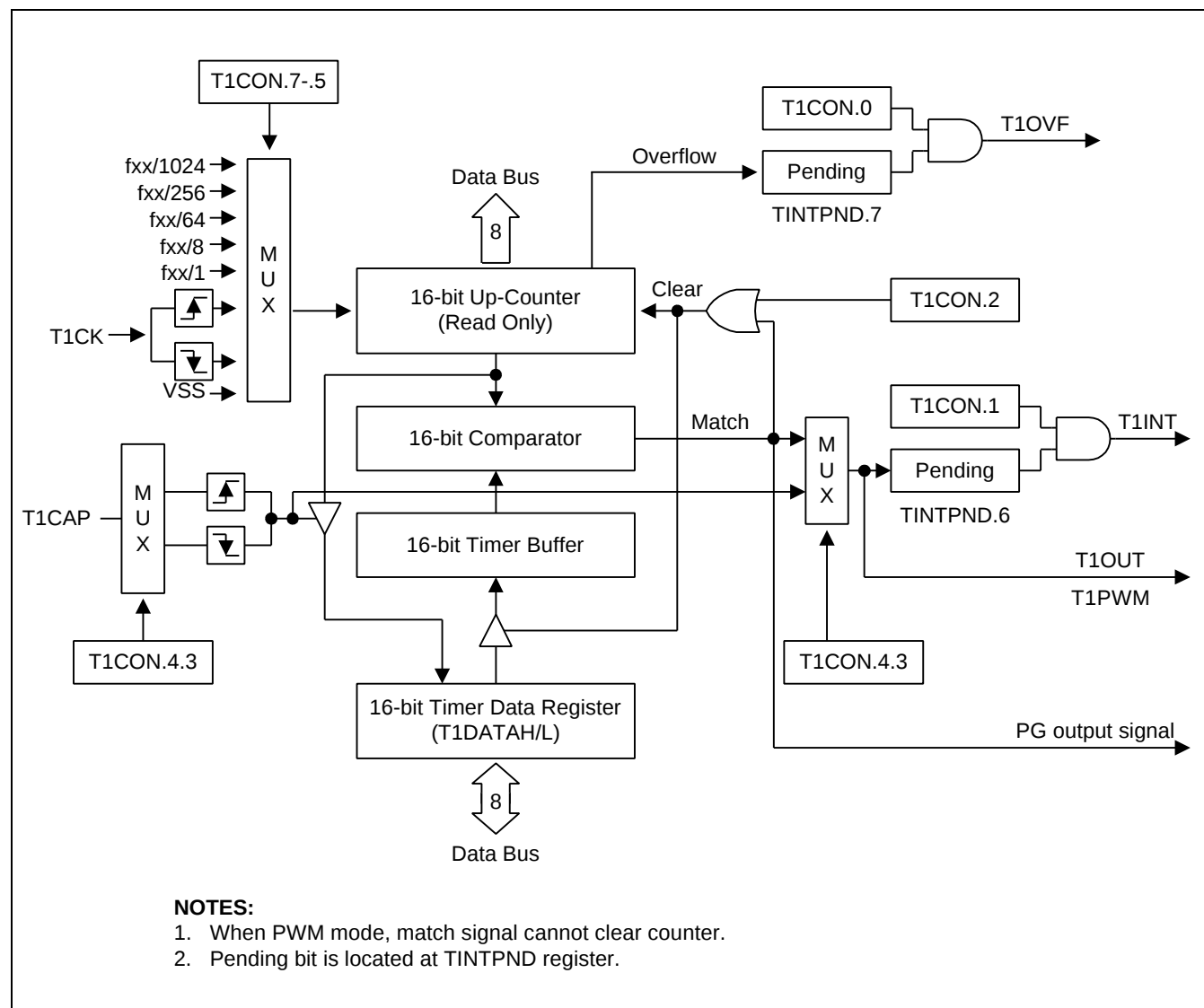
Figure 12-3. TIMER 1 Functional Block Diagram
