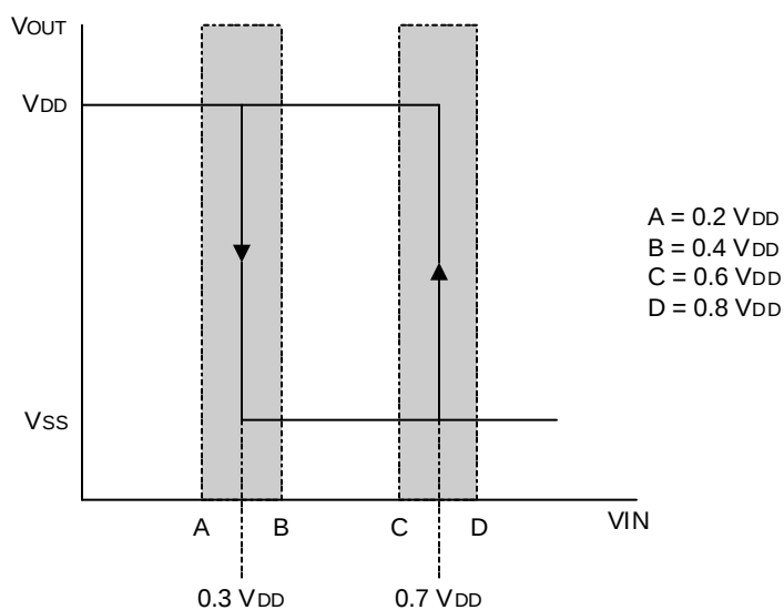
Figure 18-3. Schmitt Trigger Input Characteristic Diagram
