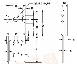
TO-247 (3P)
