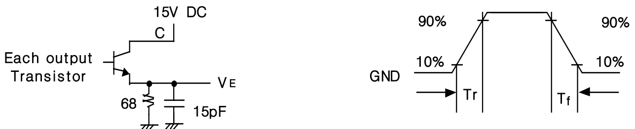
Fig. 4 Emitter-Follower Configuration Test circuit and waveform Voltage waveform
