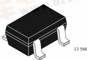
S504TRW Marking: W04 Plastic case (SOT 343R) 1 = Source, 2 = Drain, 3 = Gate 2, 4 = Gate 1
