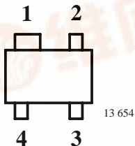
S504TRW Marking: W04 Plastic case (SOT 343R) 1 = Source, 2 = Drain, 3 = Gate 2, 4 = Gate 1
