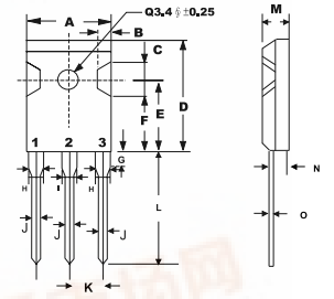
TO-247 (3P)
