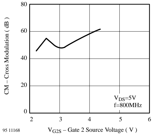
95 11168 V_{G2S} - Gate 2 Source Voltage ( V ) Figure 8. Cross Modulation vs. Gate 2 Source Voltage
