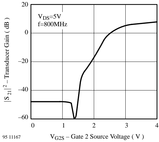
95 11167 V_{G2S} - Gate 2 Source Voltage ( V ) Figure 7. Transducer Gain vs. Gate 2 Source Voltage
