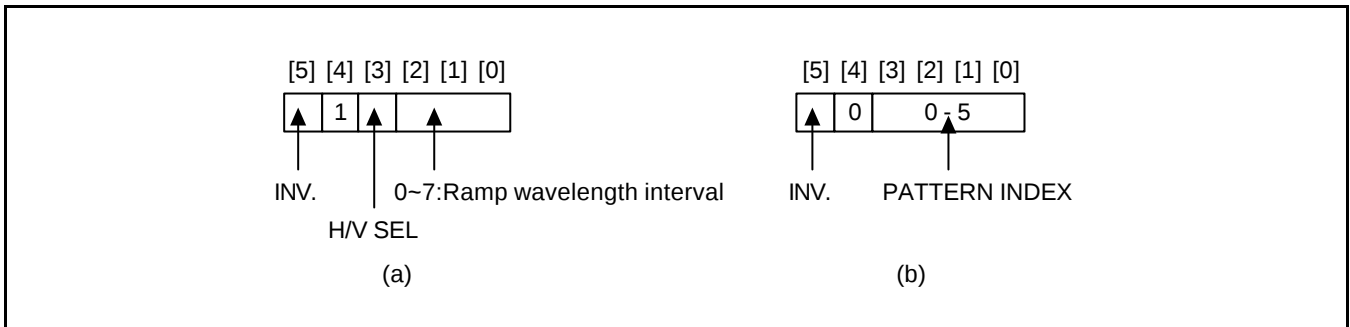
Figure 21. Test Pattern Generation Method
