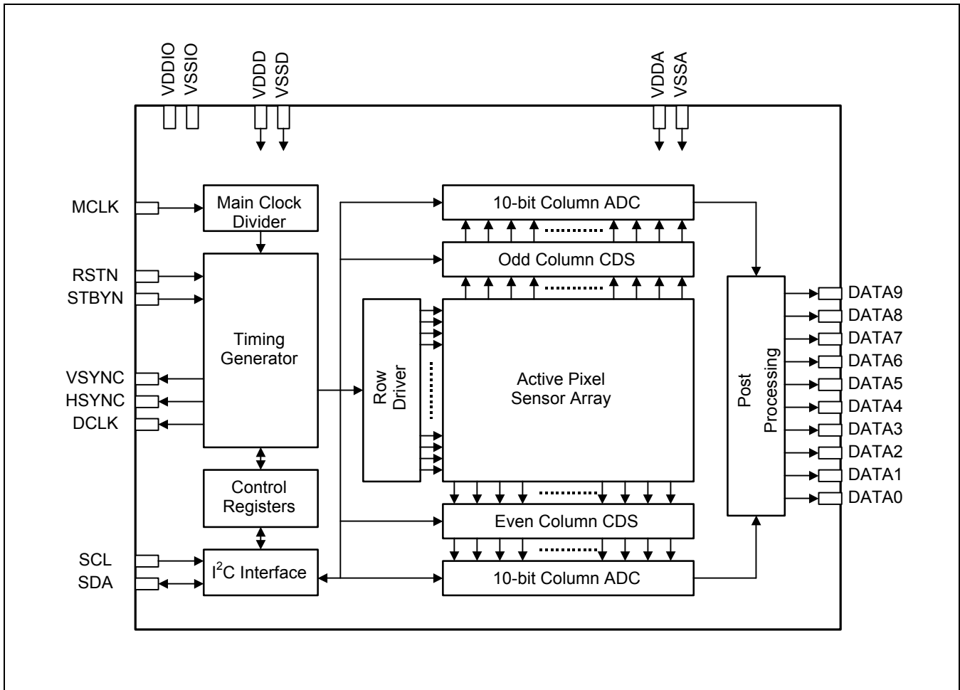
Figure 1. Block Diagram
