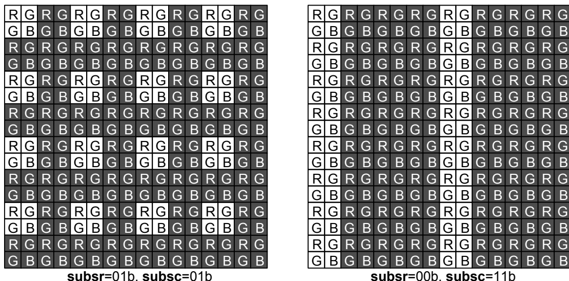
Figure 5. Bayer Space Sub-Sampling Examples
