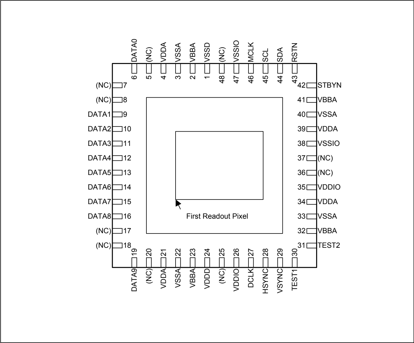
Figure 3. Pin Configuration
