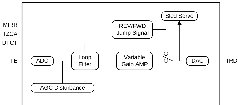
Tracking Servo Block Diagram
